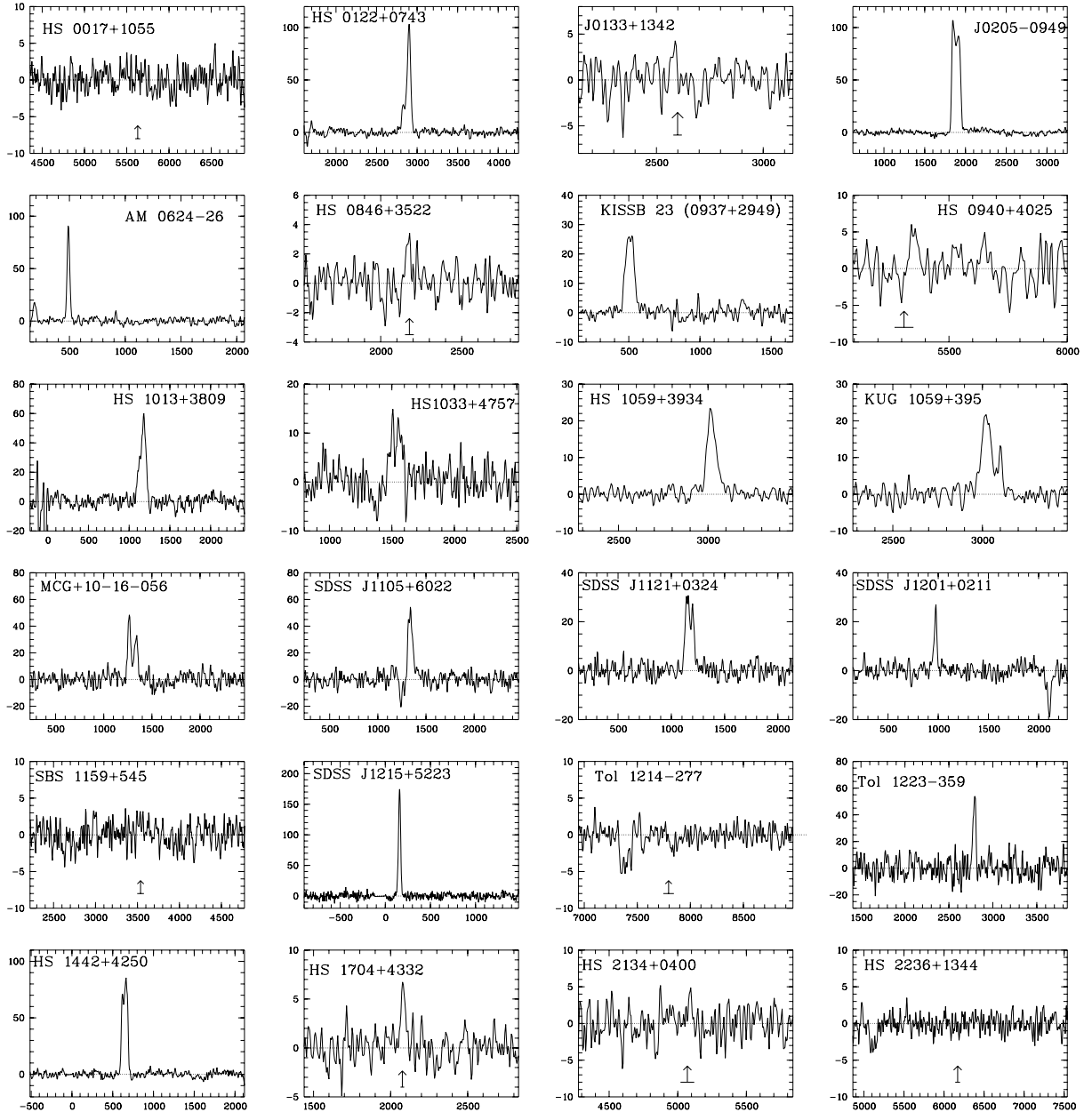
Fig. 1. The NRT HI profiles S_\nu (in mJy) vs. V_{\text{hel}} ( \text{km s}^{-1} ) of all studied galaxies with the resolution of 10.5 \text{ km s}^{-1} . The vertical arrows at the bottom with the horizontal bars show the optical velocity and its \pm 1\sigma uncertainty for weak detections or non-detected objects.
