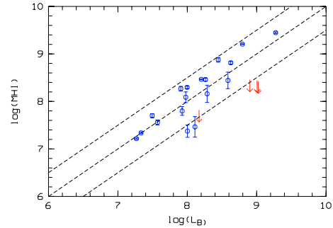
Fig. 2. Relation between M(\text{H I}) and L_B for the XMD galaxies from this paper. Middle dashed line corresponds to positions of objects with M(\text{H I})/L_B = 1.0 , while the upper and lower lines for objects with this ratio equal 3 and 1/3 , respectively. The arrows show the upper limits on M(\text{H I}) .
