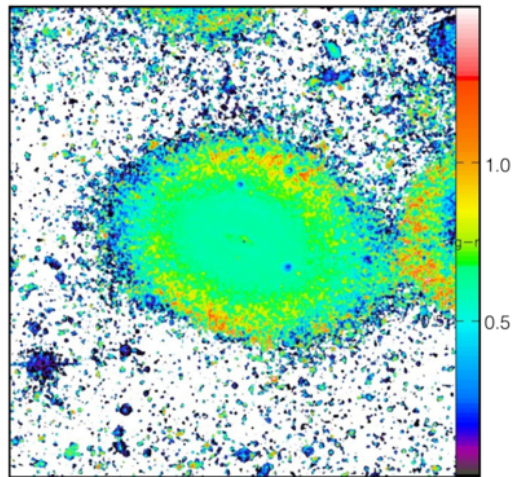
Figure 8. g-r colour map of the galaxy NGC 3489. The reddening by 0.5 mag in the outer annulus is most likely due to the internal reflection of the red galaxy nucleus. The scale in mag is shown to the right.
