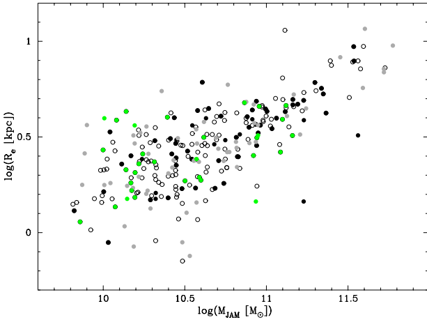
Figure 13. Selected ETGs in this catalog plotted on a diagram showing the dynamical mass, M_{JAM} , derived from modeling of the stellar kinematics and the isophotal structure of each galaxy versus the effective radius, R_e (see Cappellari et al. 2013). Open circles correspond to the full ATLAS 3D sample, and filled discs are galaxies with available deep imaging (grey ones belong to Virgo and were not analyzed here). Relaxed galaxies showing no sign of tidal perturbations even with the deep imaging are shown in green.
