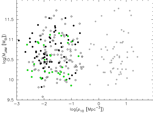
Figure 12. Selected ETGs in this catalog plotted on a diagram showing the dynamical mass, M_{JAM} , derived from modeling of the stellar kinematics and the isophotal structure of each galaxy, versus the volume density diagram, \rho_{10} , in \log (Mpc^{-3}) . Open circles correspond to the full ATLAS 3D sample, and filled discs are galaxies with available deep imaging. Note that all galaxies located in regions with density above \log(\rho_{10}) = -0.4 belong to the Virgo Cluster and were observed as part of the NGVS project (filled grey discs). They will be presented in a separate paper. Relaxed galaxies showing no sign of tidal perturbations even with the deep imaging are shown in green.
