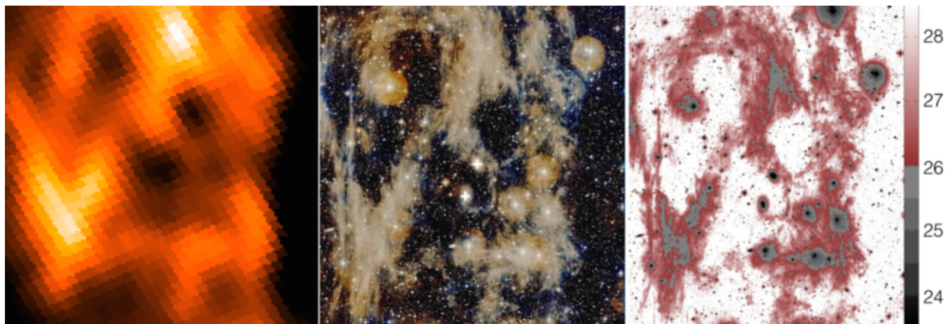
Figure 9. Contamination by Galactic cirrus. Middle: Composite g+r MegaCam image of the field around NGC 2592 and NGC 2594. The position of each ETG is indicated by the white cross. The field of view is 51 \times 57 arcmin. Left: The same field observed by the HFI camera on board Planck at 857 GHz ( 350 \mu\text{m} ). Note the very good match between the extended emission in the far IR and the optical, though the MegaCam image has a spatial resolution which is 300 times better than HFI. Right: Surface brightness map in the g-band. The scale in \text{mag arcsec}^{-2} is indicated to the right. Note that most cirrus emission shows up at surface brightness below 26 \text{ mag arcsec}^{-2} (shown in red).
