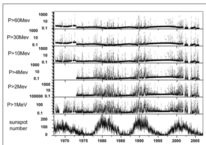
Figure 1. (top to bottom) Total proton flux (P) (solar and cosmic origin) above various energy levels and solar activity (daily sunspot number) for four solar cycles.
