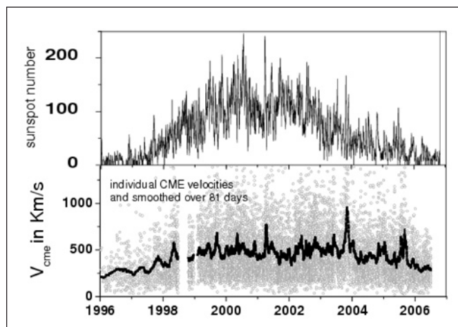
Figure 2. (top) Sunspot number as a function of time. (bottom) Coronal mass ejection velocity as a function of time. Individual coronal mass ejections are shown as gray circles, and the 81-day smoothed values are represented by the solid curve.
