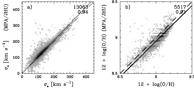
Figure 10. Comparison of (a) the velocity dispersions and (b) the oxygen abundances determined by the MPA/JHU group with our estimates. The solid line shows a y = ax + b linear fit to the data, while the dashed one is the identity line ( y = x ).
