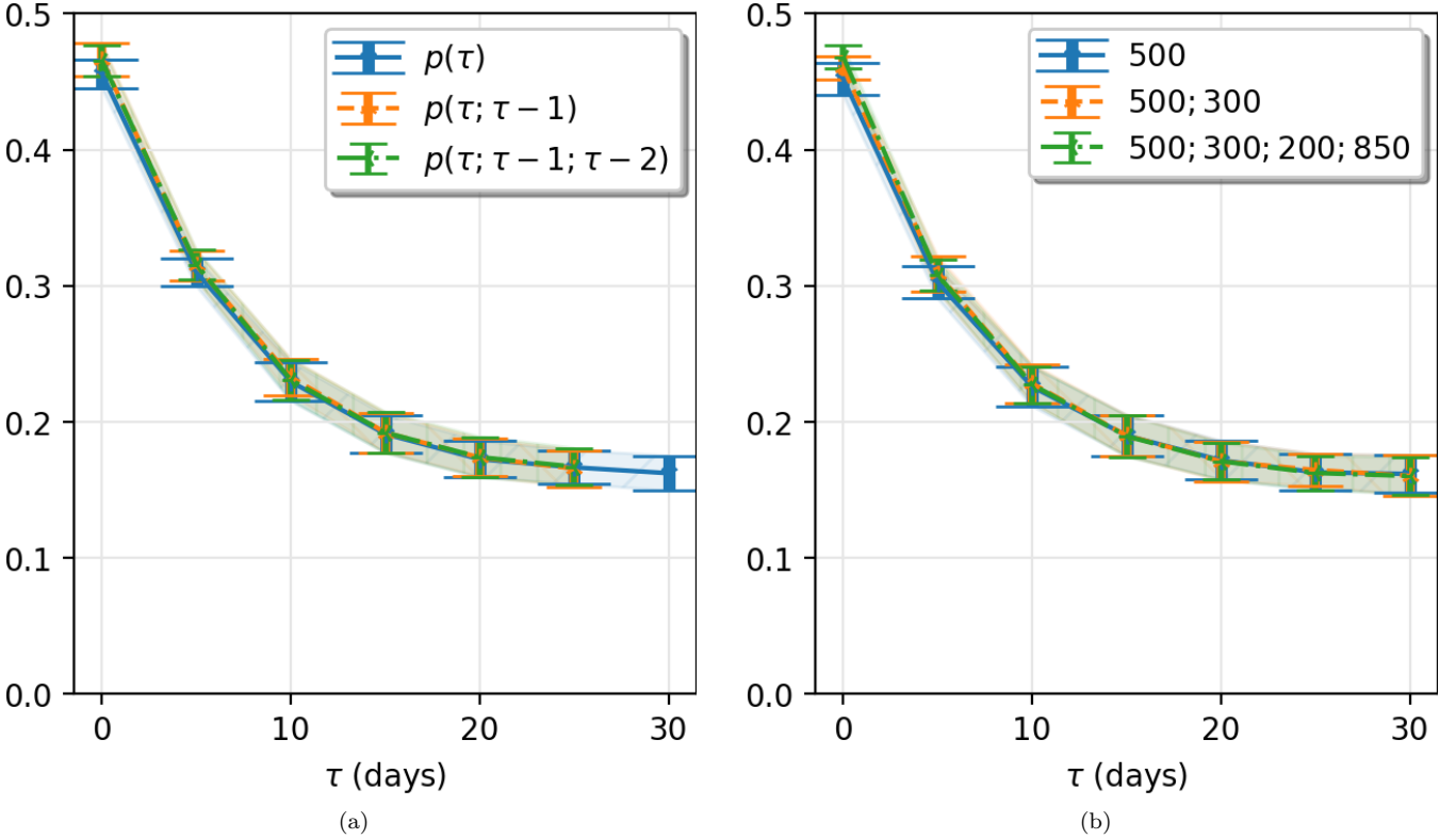
FIG. 6. Prediction skills when training the network with extra fields. The Normalized Logarithmic Score is on the y -axis. Panel (a) Addition of stacked fields at extra time steps: (T_F, Z_{NH}, S_F)(t-\tau) (blue), [(T_F, Z_{NH}, S_F)(t-\tau), (T_F, Z_{NH}, S_F)(t-\tau-1)] (orange), [(T_F, Z_{NH}, S_F)(t-\tau), (T_F, Z_{NH}, S_F)(t-\tau-1), (T_F, Z_{NH}, S_F)(t-\tau-2)] (green). The NLS features a very small improvement when adding the previous day information, but none if we add two previous days. (b) Addition of extra levels of geopotential height [T_F, Z_{NH}(500hPa), S_F] (blue), [T_F, Z_{NH}(500hPa), Z_{NH}(300hPa), S_F] [T_F, Z_{NH}(850mbar), Z_{NH}(500hPa), Z_{NH}(300hPa), Z_{NH}(200hPa), S_F] (green). The NLS features a very small improvement, although not statistically significant, when adding more geopotential height fields.
