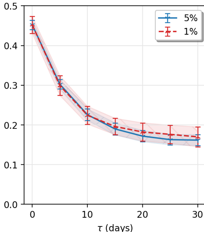
FIG. 12. Benchmarks for the optimal Normalized Logarithmic Score obtained by the proposed neural network for 5 percent heatwaves (blue) and 1 percent heatwaves (red)
