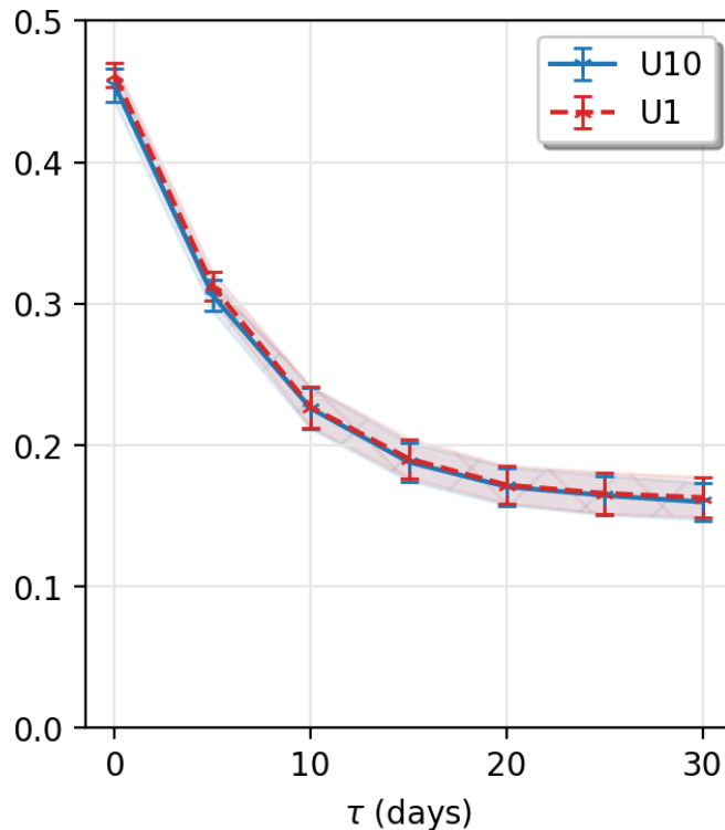
FIG. 11. Normalized Logarithmic Score versus lead time \tau for a neural network trained with the (T_F, Z_{NH}, S_F) predictors, with undersampling with r = 10 (U10) (blue), and without undersampling (U1) (red). The two skill curves are within error bars of the experiment.
