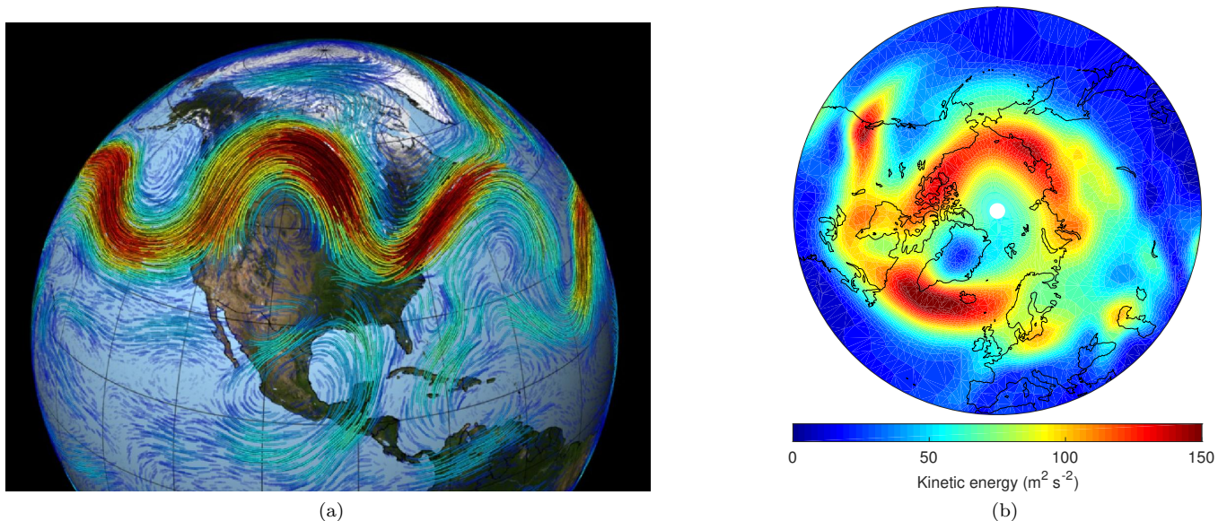
FIG. 1. (a) Snapshot of wind speed velocity at the top of the troposphere, showing the jet stream over North America (from NASA). (b) Averaged horizontal kinetic energy at 500hPa (mid troposphere) in the PlaSim model [67], showing the averaged Northern Hemisphere jet stream
