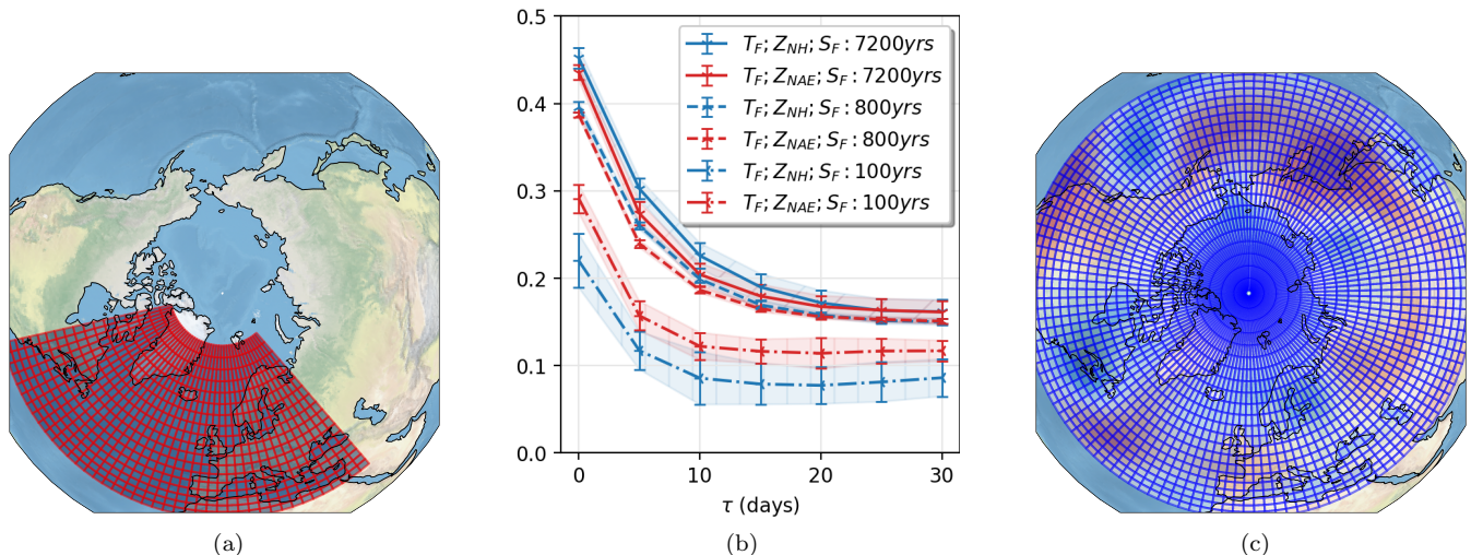
FIG. 7. Prediction skills versus dataset lengths and optimal geographical area. Panels a) and c) show PlaSim grid for the North Atlantic and Europe sector (NAE,a), and Northern Hemisphere mid and high latitude sector (NH,c), respectively. Panel b): Normalized Logarithmic Score versus lead time \tau , for neural networks trained with (T_F, Z_{NH}, S_F) predictors (blue) and (T_F, Z_{NAE}, S_F) predictors (red), and with datasets of length 7,200 years (plain lines), 800 years (dashed lines) and 100 years (dashed-dotted lines). The results illustrate the lack of data regime, with very slow convergence of the prediction skill with the dataset length, and with a clear tradeoff between dataset length and size of optimal geographical area for best prediction.
