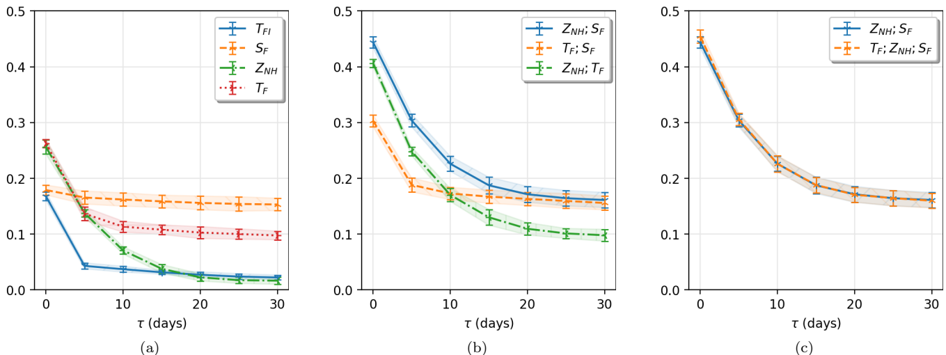
FIG. 5. Relevant climate fields for best prediction: All figures show the Normalized Logarithmic Score (NLS) (cf. equation (6)), versus the lead time \tau , for different combinations of the predictor fields. Fields are either integrated over the area of France (FI), masked over the France area (F) or over the Northern Hemisphere (NH). From k -fold cross-validation values, we plot the averaged NLS, plus or minus one standard deviation (shaded area and error bars): (a) Single field prediction: T_{FI} (blue), S_F (orange), Z_{NH} (green), and T_F (red) ; (b) Fields combined pairwise for prediction: (Z_{NH}, S_F) (blue), (T_F, S_F) (orange), (Z_{NH}, T_F) (green), ; (c) All three fields combined for prediction: (T_F, Z_{NH}, S_F) (orange).
