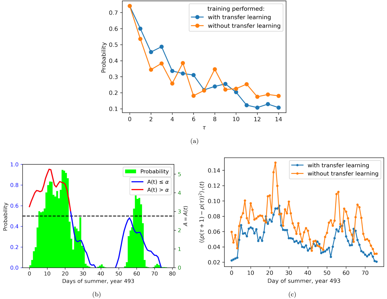
FIG. 10. (a) Evolution of the committor function along a trajectory p[X(t^* - \tau), \tau] as a function of lead time \tau , for a prediction of a potential heatwave at a prescribed physical time t^* . The orange points show the committor learned independently for each \tau , while the blue ones are obtained with transfer learning from one \tau to the next. (b) Illustration of the A(t) (blue/red line) and p[X(t), 0] (in green) trajectories during summer of a specific year; red line corresponds to moments where the actual A = A(t) > \alpha (see equation (1)), above 95 percentile threshold, while blue line denotes that A = A(t) \leq \alpha . The filled green segments show the probability predicted by the neural network trained on T_F, Z_{NH}, S_F . This plot illustrates the general correlation between A = A(t) \leq \alpha and T_F, Z_{NH}, S_F . (c) Display of \sigma_\tau(t) , as defined in equation (10), for the same year as in (b), for the method with transfer learning (in blue) and without (in orange). We see that the latter is almost always above. This illustrates that variance between subsequent points is larger when transfer learning is not applied.
