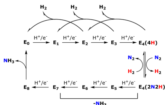
Figure 6 | Modified Lowe-Thorneley model for N 2 reduction by Mo-dependent nitrogenase. The E n labeling indicates n number of proton and electron pairs that have been loaded on one of the αβ-dimers of NifDK. Reprinted (Adapted or Reprinted in part) with permission from ref. 51 . Copyright 2020 American Chemical Society.
