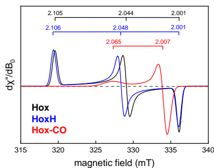
Figure 31 | EPR spectra of the oxidized H-cluster. Simulations of EPR spectra for the oxidized states H ox , H oxH , and H ox-CO as observed in CrHydA1 . The g-values are indicated. Reprinted (Adapted or Reprinted in part) with permission from ref. 267 . Copyright 2020 American Chemical Society.
