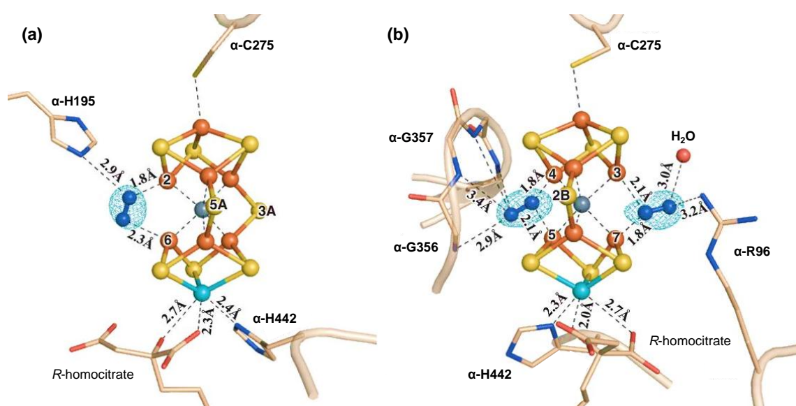
Figure 12 | Crystal structure of NifDK*. The M-cluster and key interacting residues at Site 1 (a) and Site 2 (b) are depicted (PDB ID 6UGO). The cluster and N molecules are presented
