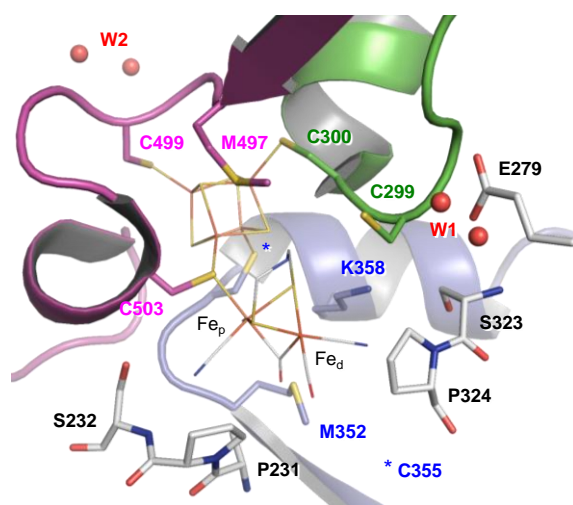
Figure 30 | Active site cavity and catalytic cofactor of [FeFe]-hydrogenase CpI. The H-cluster is comprised of an [4Fe-4S] cluster and the diiron site (PDB ID 4XDC). Loop 1–3 provide four cysteine residues to bind the [4Fe-4S] cluster and the diiron site. In loop 1
