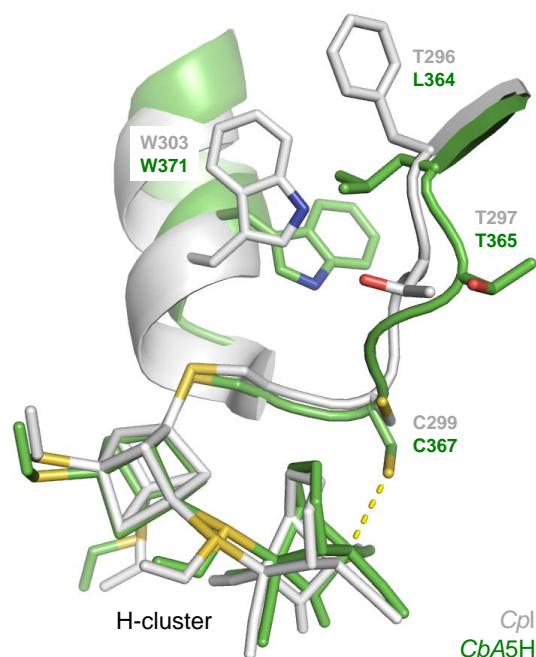
Figure 35 | Comparison of CpI (white) and CbA5H (green) in the H_{\text{ox}} and H_{\text{inact}} state. The distance of the sulfur atom of C299/C367 shrinks from \sim 6 Å to \sim 3 Å, making a direct coordination of the distal iron ion ( Fe_d ) in the H_{\text{inact}} state of CbA5H likely (dashed line). The annotated amino acid residues have been identified to cause the flexibility of the unique loop in CbA5H . Drawn after PDB IDs 4XDC and 6TTL.
