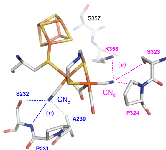
Figure 36 | Hydrogen-bonding environment of the CN - ligands. In proximal (p) position, polar interactions ( \nu ) with a backbone amine, S232, and variant A230S have been experimentally verified in CpI and CrHydA1 . The hydrophilic pocket including K358, S323, and a P324 backbone contact inspired the assignment of the CN - ligand in distal (d) position in CpI and DdH . The putative hydrogen-bonding environment ( \nu ) is shown. Drawn after PDB ID 6NAC. Atomic coloring: Fe, orange; S, yellow; C, gray; O, red; N, blue.
