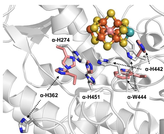
Figure 10 | Crystal structure of \Delta nifB NifDK (PDB ID 1L5H). The M-cluster and selected residues included from wild-type A_v NifDK are overlaid (in pink; PDB ID 3U7Q). The two structures were aligned, and the M-cluster and specific residues from the wild-type protein were superimposed on top of the \Delta nifB NifDK structure. The residues \alpha -H274, \alpha -H442, and \alpha -H451 represent the identified ‘histidine triad’. The cluster atoms are shown as ball-and-stick models, and the amino acid residues are represented as sticks. Atomic coloring: Fe, orange; S, yellow; C, gray; O, red; N, blue.
