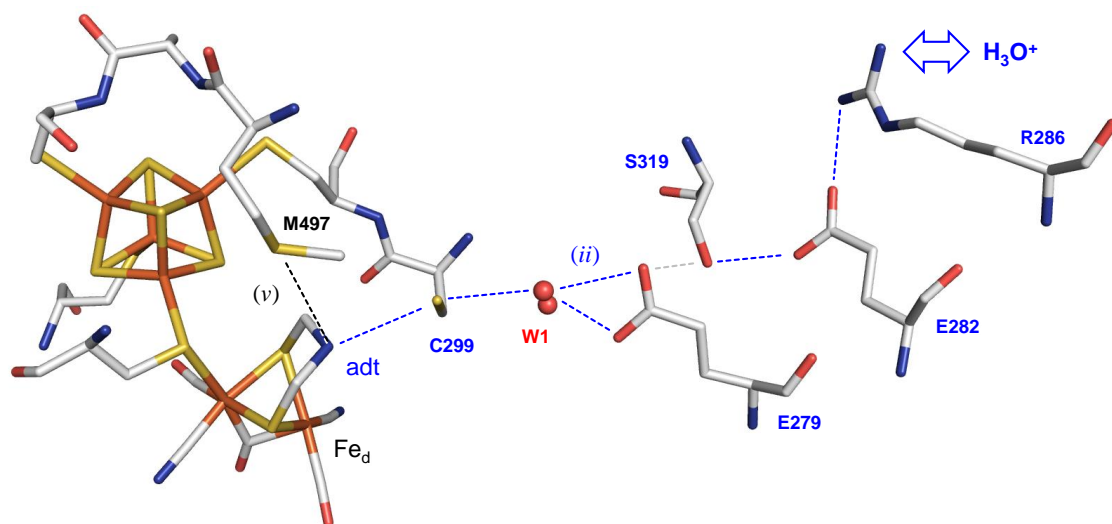
Figure 38 | The ‘catalytic’ proton transfer pathway in [FeFe]-hydrogenase CpI . The sidechain of M497 may stabilize the orientation of the ADT ligand by a hydrogen bond (v). Dashed blue lines represent the hydrogen-bonding network (ii) of the proton transfer pathway. Note that a bond between E279 and S319 is unlikely in the oxidized state (dashed grey line) but likely formed upon reduction and protonation of the cofactor. Drawn after PDB ID 4XDC. Atomic coloring: Fe, orange; S, yellow; C, gray; O, red; N, blue.
