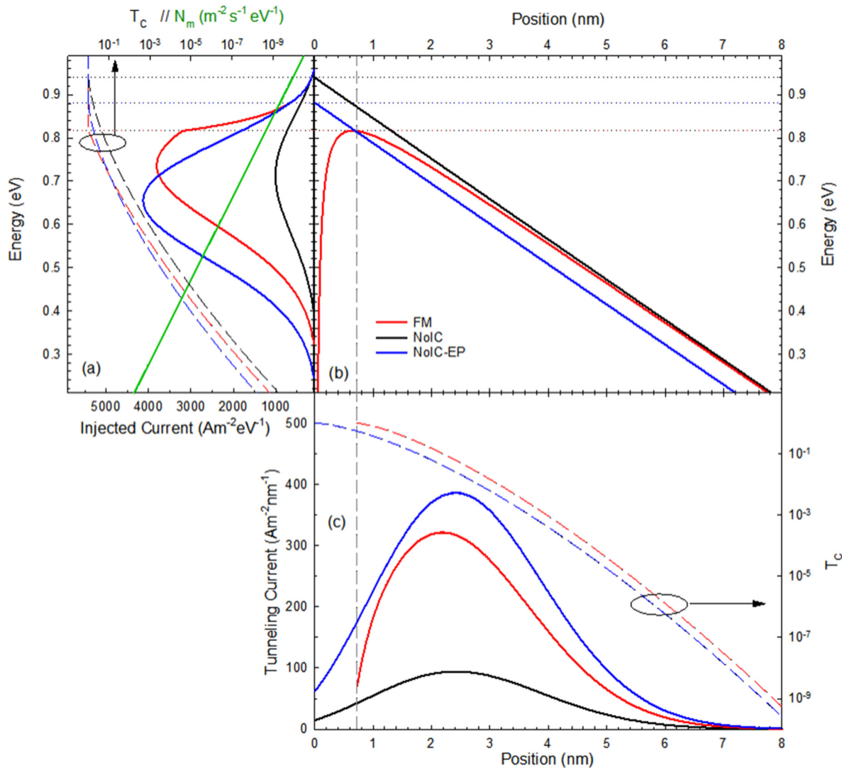
FIG. 5. Comparison of three case studies for T = 475 \text{ K} and V = -20 \text{ V} : (i) including IC (FM, red lines), (ii) without IC and using the same parameters as the FM (NoIC, black lines) and (iii) without IC but using the effective parameters (NoIC-EP, blue lines). (a) Injected current (solid lines), transmission coefficient (dashed lines), and rate of electrons incident on the barrier [Eq. (6), green line] as a function of energy; (b) conduction band and (c) tunneling current (solid lines) and transmission coefficient (dashed lines) as a function of the distance from the metal–semiconductor interface. The horizontal dotted lines in (a) and (b) indicate the top of the barrier in each case, i.e., the energy separating tunneling and thermionic injection. The vertical dashed line in (b) and (c) indicates the position of the maximum of the barrier in the FM case.
