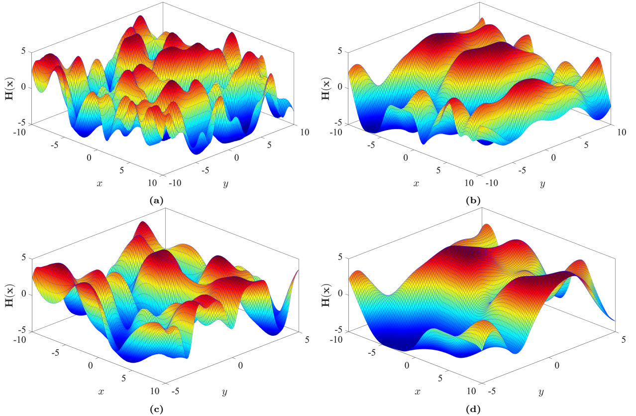
Fig. 5. 2D interval field realisations with H_c = 0 , H_r = 5 and (a) \Omega = [-10, 10]^2 and R_{dx} = R_{dy} = 2 ; (b) \Omega = [-10, 10]^2 and R_{dx} = 5 , R_{dy} = 2 ; (c) \Omega = [-10, 10] \times [-5, 5] and R_{dx} = R_{dy} = 2 ; (d) \Omega = [-10, 10] \times [-5, 5] and R_{dx} = 5 , R_{dy} = 2 .
