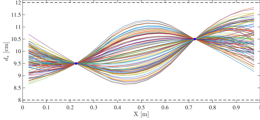
Fig. 16. A hundred realisations of cross-sectional diameter with two deterministic local values.
