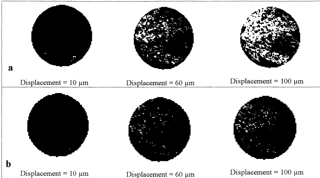
Fig. 2. — a) Evolution of the contact area with the normal stress (simplistic model). b) Evolution of the contact area with the normal stress (Hopkins' mechanical model).
