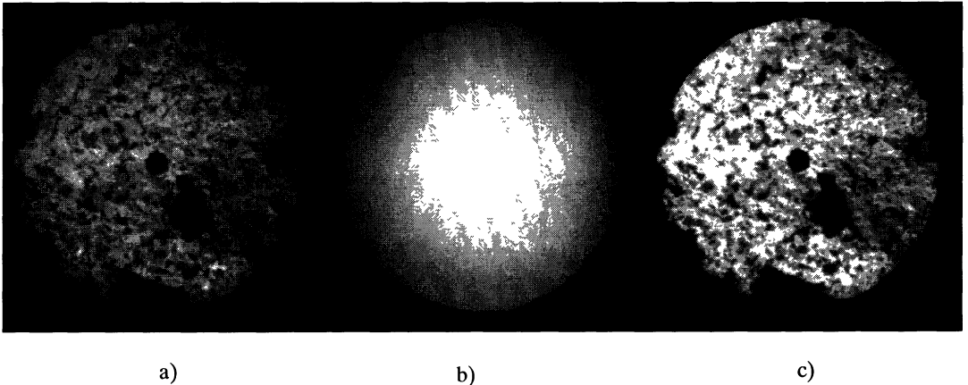
Fig. 1. — a) Grey level image of the fracture cast (one pixel = 0.448 mm × 0.300 mm). b) Halo on the light source image. c) Cast image corrected of the light source heterogeneities.
