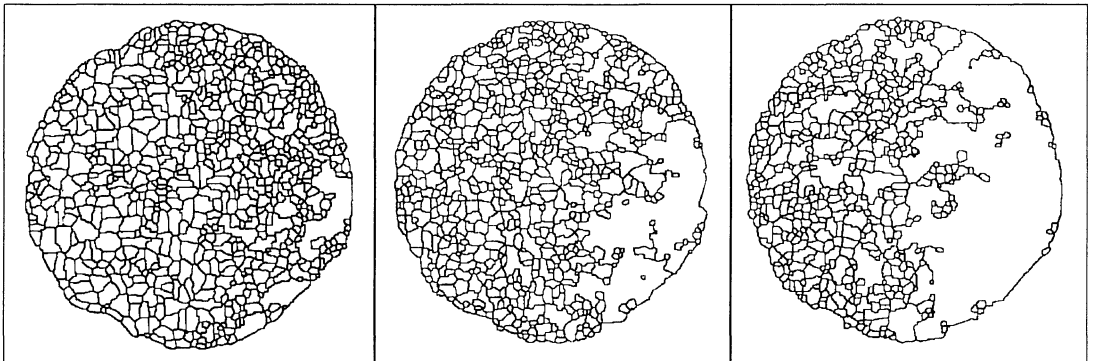
Fig. 6. — Example of evolution of a skeleton when the normal stress increases.
