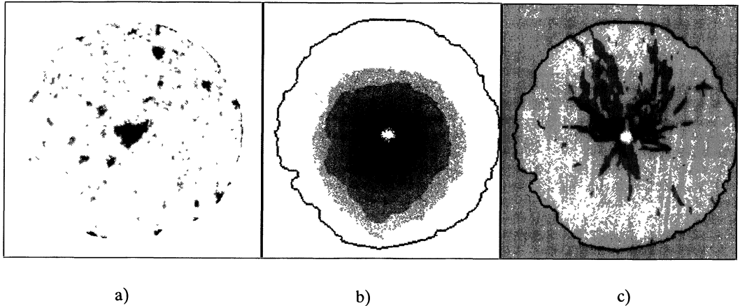
Fig. 3. — a) Cast image. b) Map of the fluid pressure in the fracture - Darker is the grey level, higher is the pressure (3FLO Model). c) Map of the flow in the fracture - Darker is the grey level, higher is the flow rate (3FLO Model).
