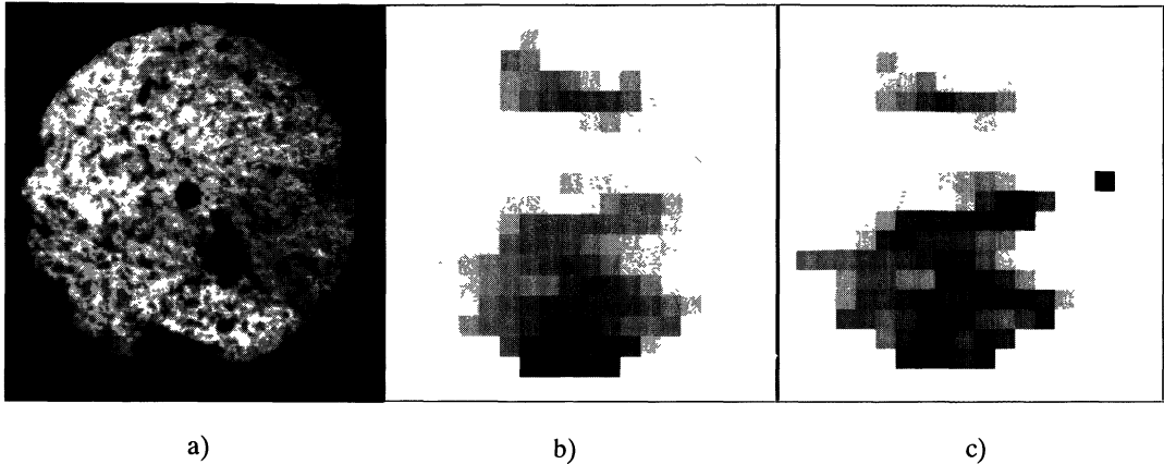
Fig. 4. — a) Cast image. b) Map of the velocity in the fracture without normal stress - Darker is the grey level, lower is the velocity (Davias' Model). c) Map of the velocity in the fracture with a lower aperture due to a normal stress - Darker is the grey level, lower is the velocity (Davias' Model). Velocities have been calculated with a low number of points (around 125).
