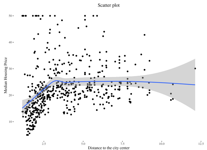
Figure 2. Scatterplot between one input and the output of the Boston housing dataset.
