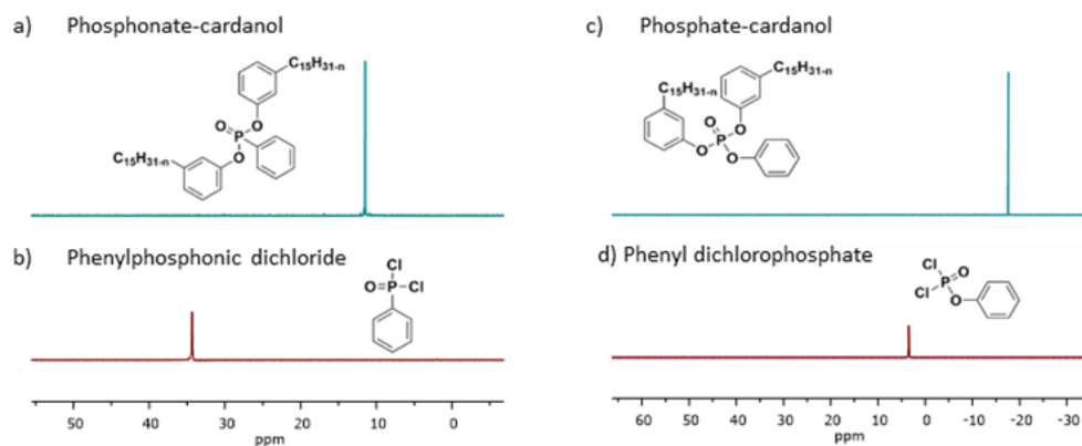
Figure 2. ^{31}\text{P} NMR spectra of phosphonate- and phosphate-cardanol compounds and their initial phosphorylated reagents.
