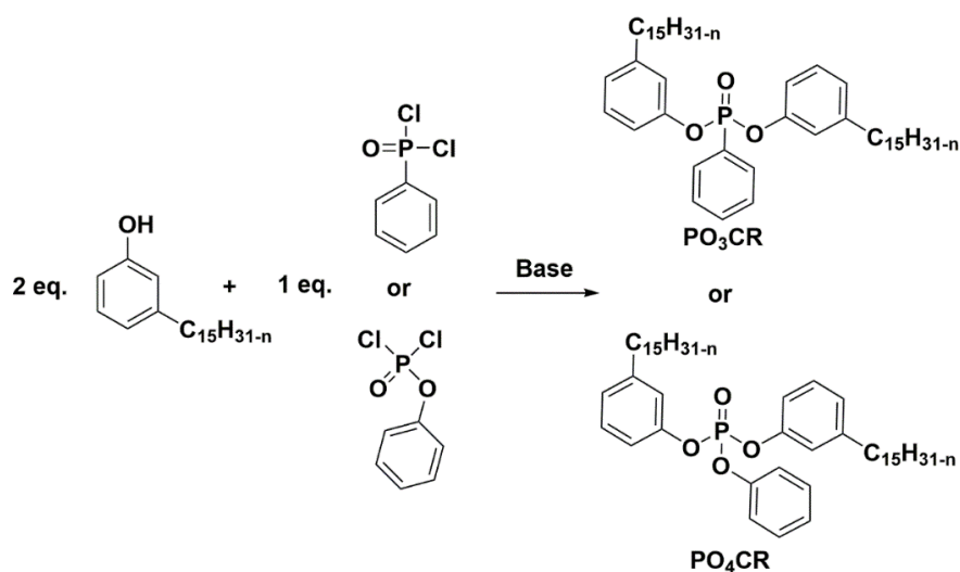
Scheme 1. General synthesis of the phosphonate- or phosphate-cardanol as reactive diluent ( \text{PO}_3\text{CR} and \text{PO}_4\text{CR} ).
