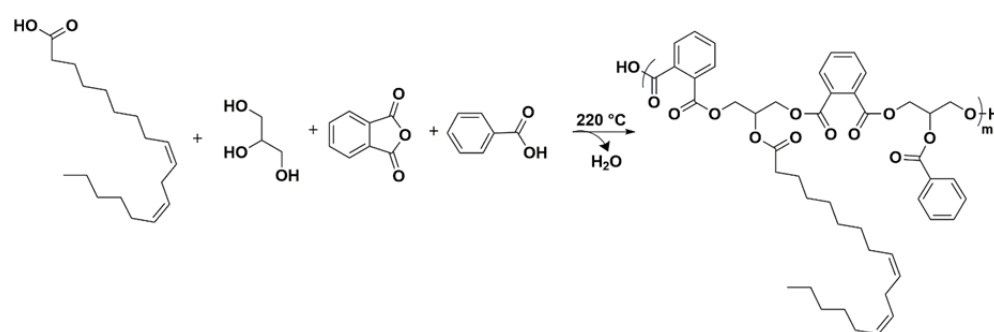
Scheme 3. Synthesis of TOFA alkyd resin.
