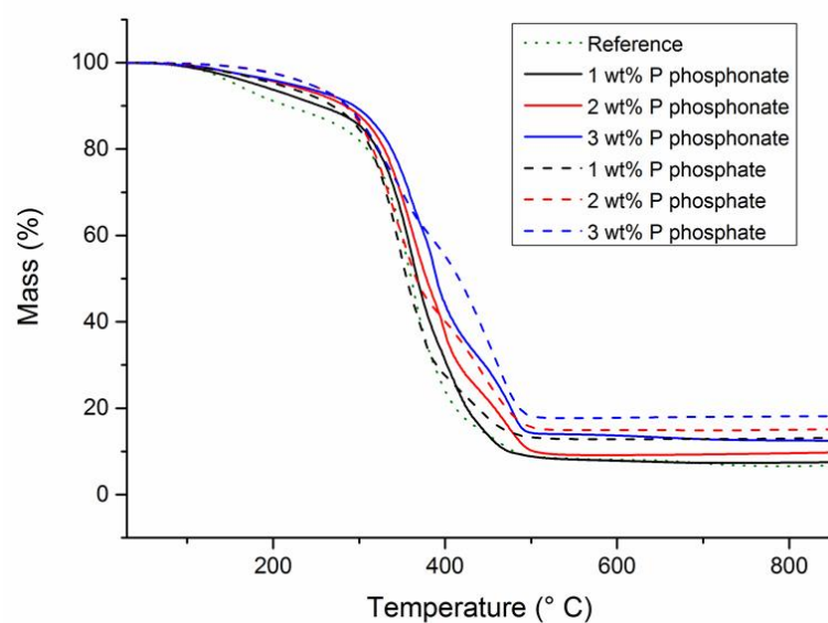
Figure 4. TGA thermograms of reference alkyd resin and phosphorylated cardanol modified alkyd resins.
