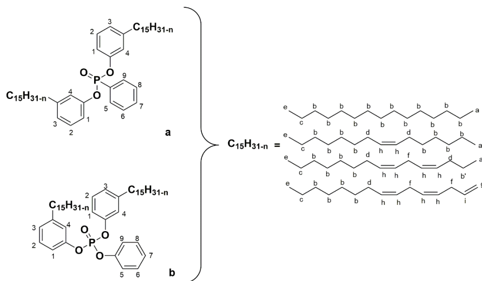
Figure 1. Structure of phosphonate- and phosphate-cardanol.
