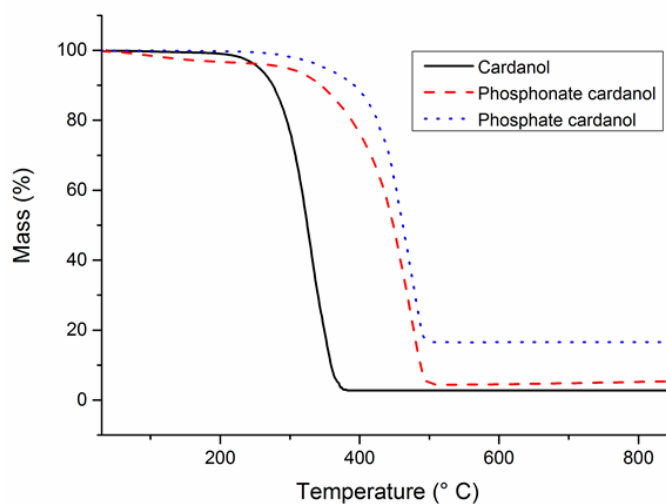
461 Figure 3. TGA thermograms of cardanol, phosphonate-cardanol and phosphate-cardanol. 462
