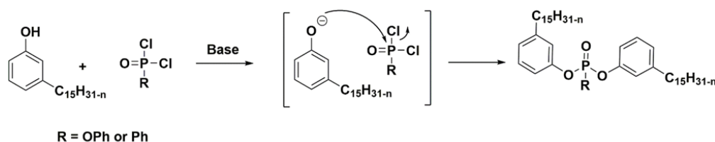
Scheme 2. Mechanism of Williamson reaction with phosphorus dichloride compounds.
