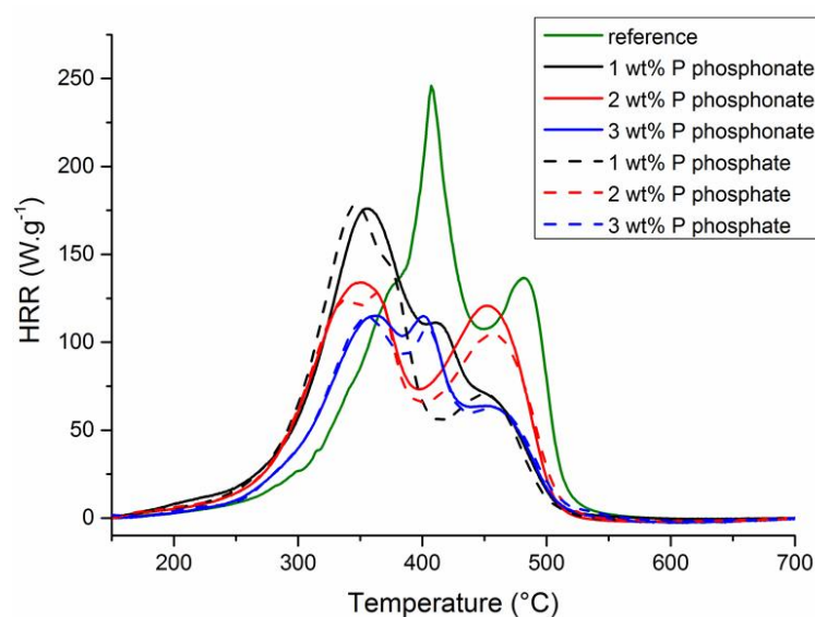
Figure 5. PCFC curves of reference alkyd resin and phosphorylated cardanol modified alkyd resins
