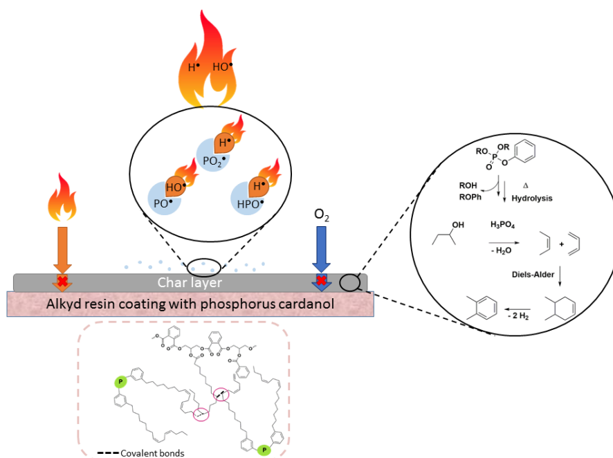
Scheme 4. Schematic illustration of possible flame retardant mechanism
