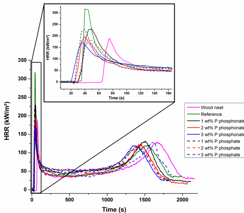
Figure 6. Curves of cone calorimeter tests for wood, reference alkyd resin and phosphorylated cardanol modified alkyd resins
