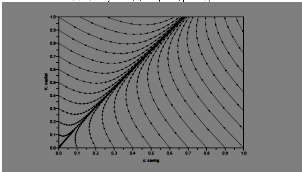
Figure 5: Situation A' Solution (s, K) of system (2) for \gamma=0.2 , \rho=0.5 , \beta=0.7 and \delta=0.3
