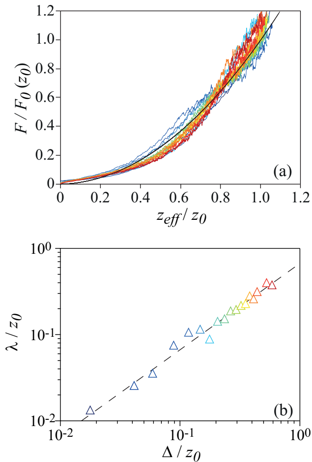
Figure 5. (a) Normalized drag force F/F_0(z_0) as a function of the normalized effective depth z_{\text{eff}}/z_0 . Color code spans from blue to red for 3 \leq \Delta \leq 100 mm respectively. The black line correspond to Eq. (3). (b) Crossover length \lambda as a function of the re-intrusion depth \Delta . The dashed line corresponds to the equation \lambda/z_0 = 0.70 \Delta/z_0 and correspond to the best fit of the data.
