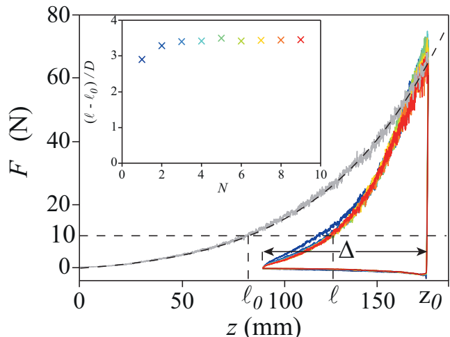
Figure 2. Drag force F experienced by a rod of diameter D = 12 mm as a function of the depth z for successive intrusion/extrusion cycles realized for z_0 = 170 mm and \Delta = 80 mm. The rod is displaced at constant velocity V_0 = 0.3 mm.s ^{-1} in glass beads of mean diameter d = 1 mm. The gray solid line corresponds to the force experienced during the first continuous intrusion. Color solid lines from blue to red represent the following nine extrusion/intrusion cycles. The dark dashed line corresponds to the best fit of the first intrusion with Eq. (1). The horizontal dash line indicates F = 10 N which intersects the force curves in \ell_0 and \ell for the first and successive intrusions respectively. Inset: (\ell - \ell_0)/D as a function of the cycle number N .
