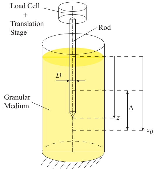
Figure 1. Sketch of the experimental setup and notations.
