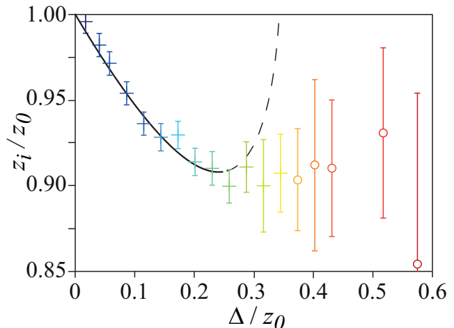
Figure 4. Normalized depth of the inflection point z_i/z_0 as a function of the normalized withdrawal distance \Delta/z_0 . The inflection points (crosses) are deduced from the re-intrusion curves presented in figure 3. The circles represent the measurements where the force curvature at z = z_r is lower than signal fluctuations and thus the determination of z_i is uncertain. The prediction of Eq. (5) for \lambda = 0.70\Delta is represented by solid line for short withdrawal distances and dashed line for large withdrawal distances.
