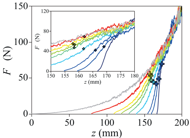
Figure 3. Drag force F on the rod as a function of the penetration depth z for different cycle amplitudes \Delta and a constant initial depth z_0 = 170 mm. Color code spans from blue to red for 3 \leq \Delta \leq 100 mm respectively. The black line represents the initial run. Inset: Zoom in of the same data around z_0 . Crosses indicate the inflection points where d^2F/dz^2 = 0 .
