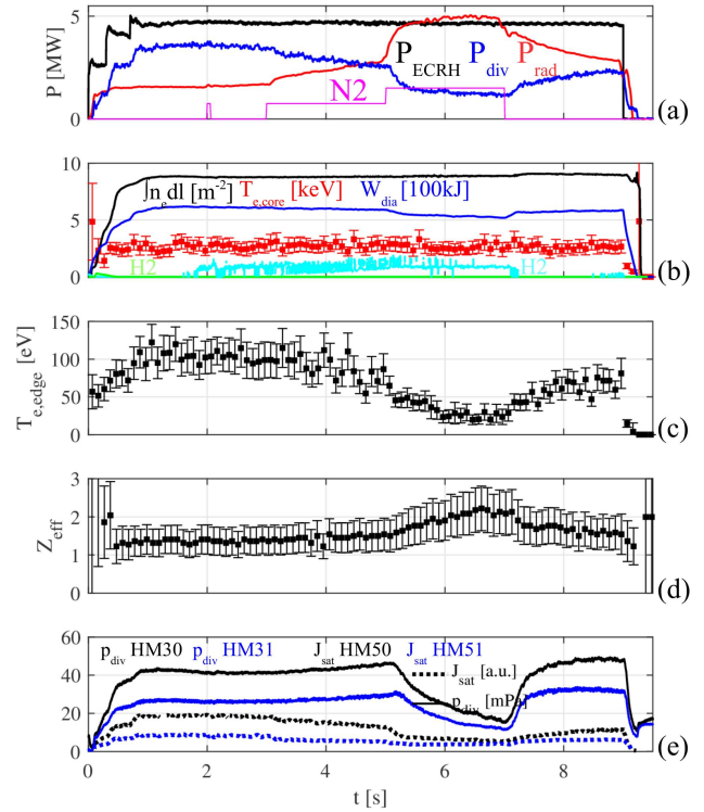
Figure 15: Time evolution of scenario with N_2 seeding (#20181016.023). (a) injected heating power (black) radiated power (red), power deposited on divertor (blue), N_2 seeding rate from gas box in HM30 (magenta) (b) line average density (black) and plasma stored energy W_{dia} (blue), core electron temperature T_{e,core} (red) from Thomson scattering (V10) near axis, H_2 fueling rates from main gas inlets (green) and HM51 divertor gas box (cyan) (c) Thomson scattering edge temperature (at the separatrix, V10), (d) effective charge state Z_{eff} , (e) neutral pressure p_{div} and local particle fluxes J_{sat} at lower (black) and upper (blue) divertor.
