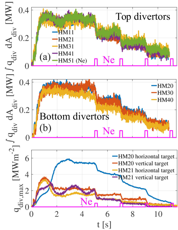
Figure 11: (a) Total top divertor heat loads. Ne seeding is performed in the HM51 divertor (green). (b) Total bottom divertor heat loads. (c) Maximum heat fluxes on horizontal and vertical targets of bottom and top divertor HM20 and HM21.
