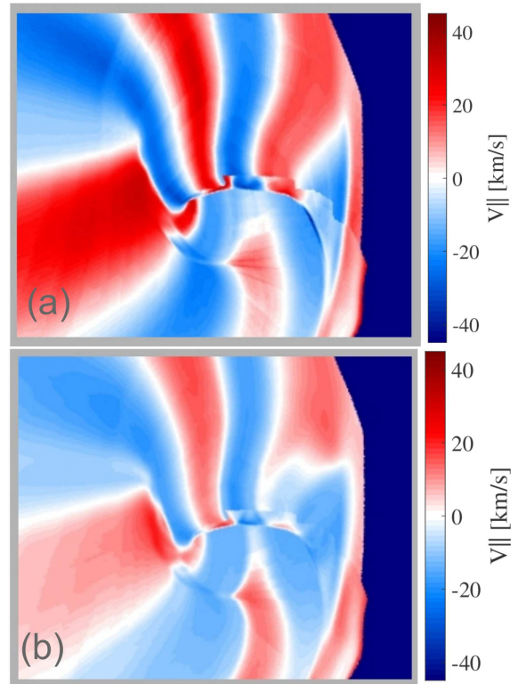
Figure 14: 3D ion flow velocities V_{||} obtained from modeling: (a) without seeding. (The box represents rotated camera view from CIS.), (b) at high Ne radiation ( \Delta P_{rad,Ne} = +2.3 MW).
