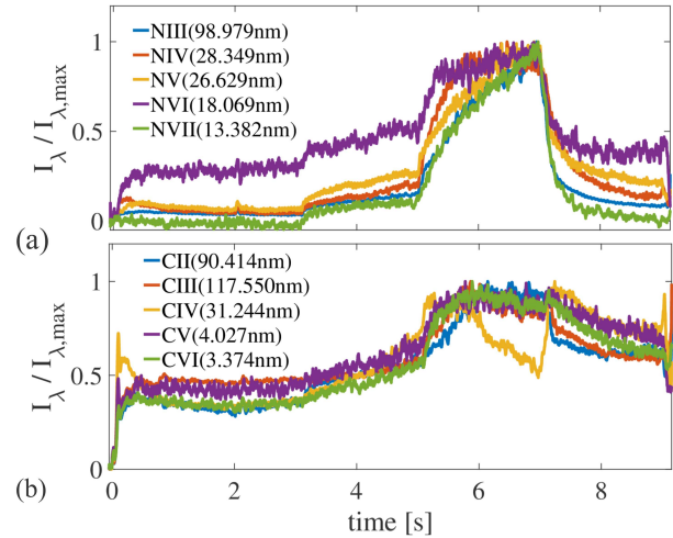
Figure 17: Overview spectrometer (HEXOS) lines for (a) nitrogen and (b) carbon. The line emission is measured at the midplane ( Z = 0 ) in the triangular symmetry plane far away from the divertor.
