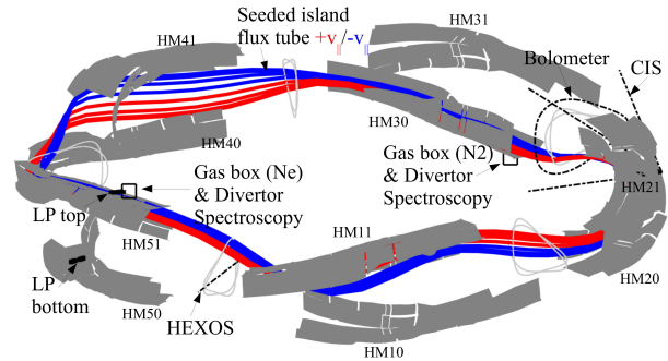
Figure 1: The geometry of the standard island divertor configuration. Full toroidal view on divertor modules and an open field line (red and blue) traced within the seeded island. Red and blue indicate the flow directions of main plasma and impurity ions.
