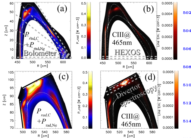
Figure 8: 3D modeling of a scenario with moderate Ne radiation. (a) Total radiated power in the triangular plane. The dashed line indicate the observation domain of the bolometer (whole poloidal plane) and HEXOS (mid plane) ( \phi = 36^\circ ) (b) CIII emission in the triangular plane. (c) Total radiated power in the divertor domain ( \phi = 12.3^\circ ). (d) CIII emission in the divertor domain. The dashed line indicate the observation of the divertor spectroscopy.
