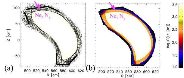
Figure 2: The geometry of the standard island divertor configuration. (a) Poincaré plot of the vacuum boundary magnetic field (standard divertor configuration). (b) Target-to-target connection lengths L_C .
