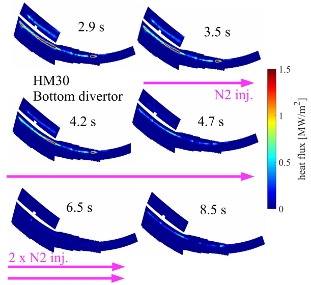
Figure 19: Bottom diverter heat loads (HM30) before, during and after N_2 injection. Asymmetric cooling: the heat flux to the vertical target reduces first and does not recover after N_2 injection.
