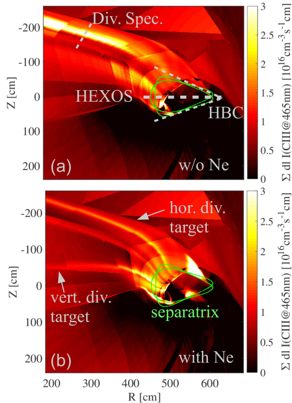
Figure 7: 3D modeling distribution of intrinsic radiation (CIII) for (a) a scenario without seeding and (b) for a scenario with Ne seeding. The dashed lines indicate the observation domain of the bolometer (whole poloidal plane in the triangular cross section), HEXOS (mid plane in the triangular cross section) ( \phi = 36^\circ ) and the divertor spectroscopy (above the horizontal target at \phi \approx 12.3^\circ ). The separatrix at the triangular cross section is shown in green.
