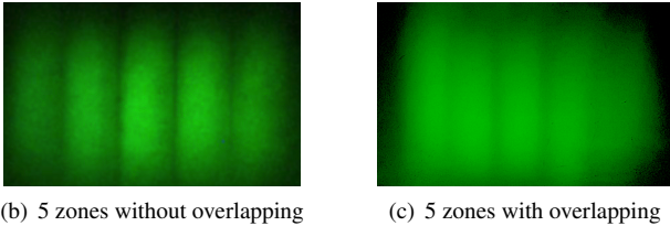
Figure 2. Observed intensity variation on a diffuse screen placed at the viewing zones. (a) The entire setting for one green laser source, where the HOE reconstructs one viewing zone. (b) The reconstruction of the 5 viewing zones at the screen for the 5 projectors, with no overlapping as in [6]. (c) The reconstruction of the 5 viewing zones with 6mm overlapping.
