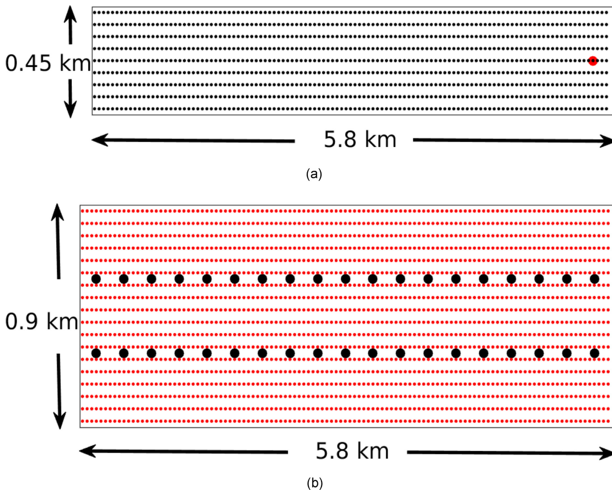
Figure 10. Acquisition geometry in the X - Y plane for a single streamer vessel (a) and ocean-bottom cables (b). The red and black dots indicate the shot and receiver locations, respectively.
