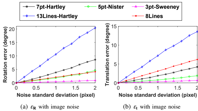
Fig. 5. Rotation and translation error with varying image noise (unit: degree). The left column reports the rotation error. The right column reports the translation error.
