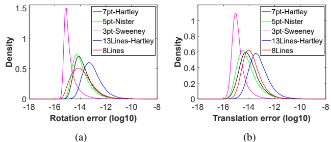
Fig. 4. Probability density functions over relative pose estimation errors in the noise-free case (100,000 runs). The horizontal axis represents the \log_{10} estimated errors and the vertical axis represents the empirical probability density. (a) reports the rotation estimation error. (b) reports the translation estimation error.
