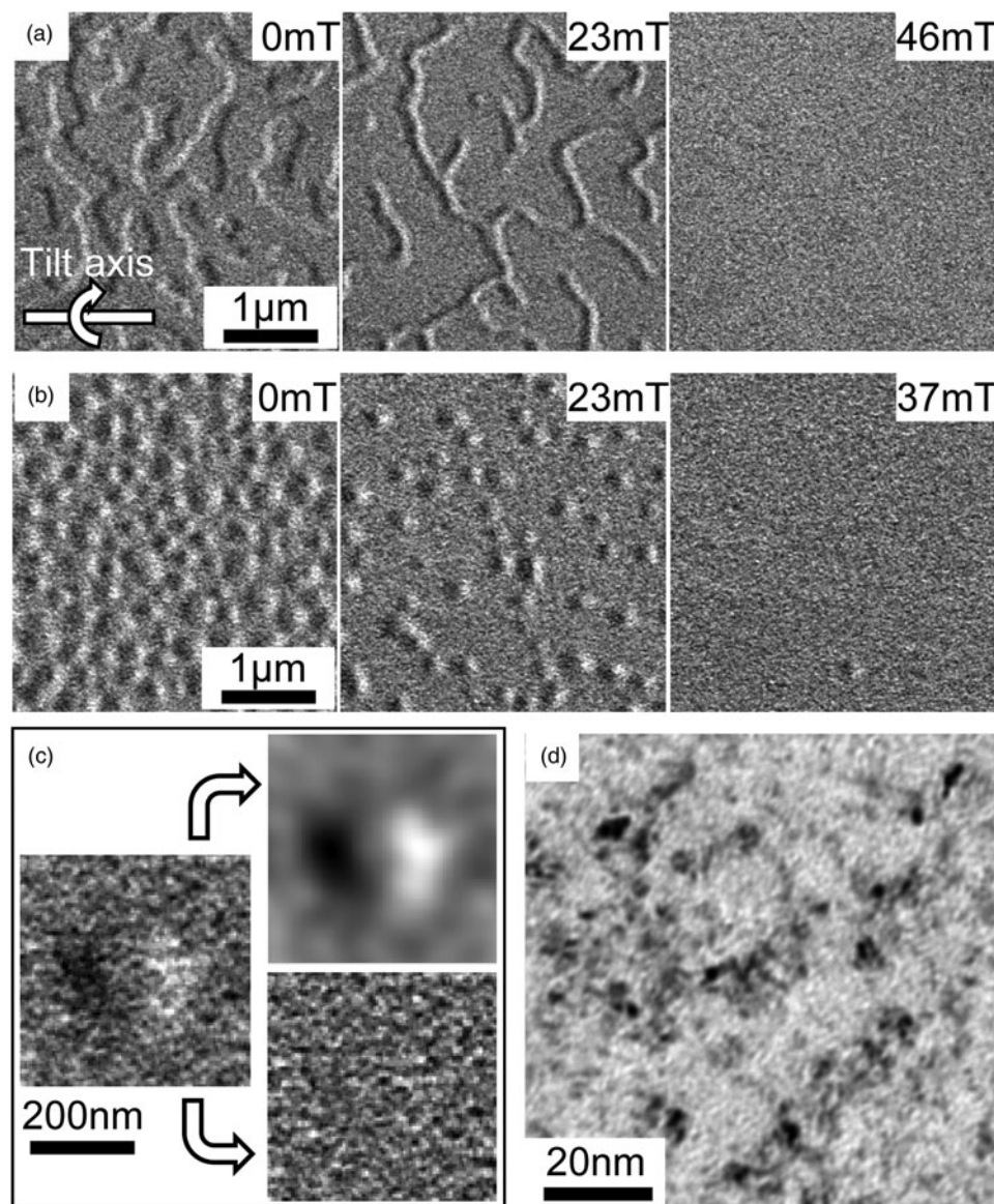
Fig. 1. (a) Fresnel defocus images of the (Pt/Co/NiFe)×5 multilayer film recorded in Lorentz mode using a defocus of -7.5 nm and a sample tilt angle of 30^\circ in the presence of the indicated magnetic fields applied using the conventional microscope objective lens. (b) Fresnel defocus images recorded after in-plane magnetic saturation of the sample in the presence of the indicated magnetic fields. (c) Left : Magnified image of a single skyrmion; Upper right : low spatial frequency components of the image; Lower right : high spatial frequency components of the image. The low and high spatial frequency components were separated using a binary circular filter of radius 10\ \mu\text{m}^{-1} in Fourier space. (d) In-focus bright-field TEM image recorded at high magnification showing the polycrystalline grain structure of the sample.
