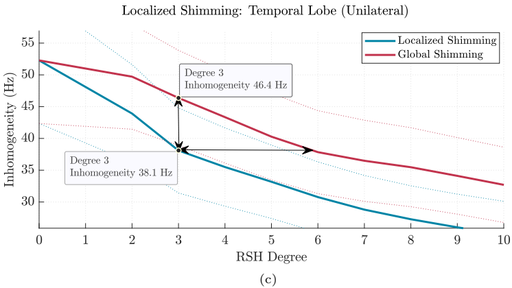
Fig. 12: Zoomed depiction of average inhomogeneity across the database in selected slabs for performance comparison between global and localized shimming techniques.
