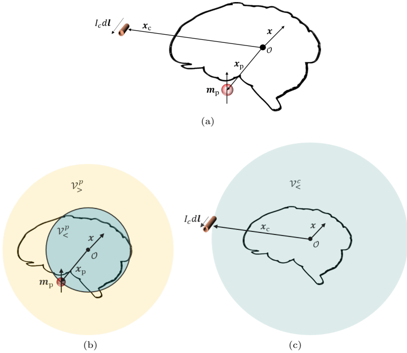
Fig. 1: (a) Disposition of fundamental building blocks for sample-induced magnetic field perturbation ( \mathbf{m}_p ) and field correction ( I_c dl ) around the brain. The MR magnet isocenter at O corresponds to the origin of the B_0 SH-decomposition. Vector \mathbf{x} \in \mathbb{R}^3 points to an arbitrary brain voxel to be shimmed. (b) A representation of the regions where the magnetic field generated by a punctual sample-induced perturbation is described by RSH ( \mathcal{V}_<^p ) and ISH ( \mathcal{V}_>^p ). (c) The region \mathcal{V}_<^c where the correction magnetic field is decomposed into RSH.
