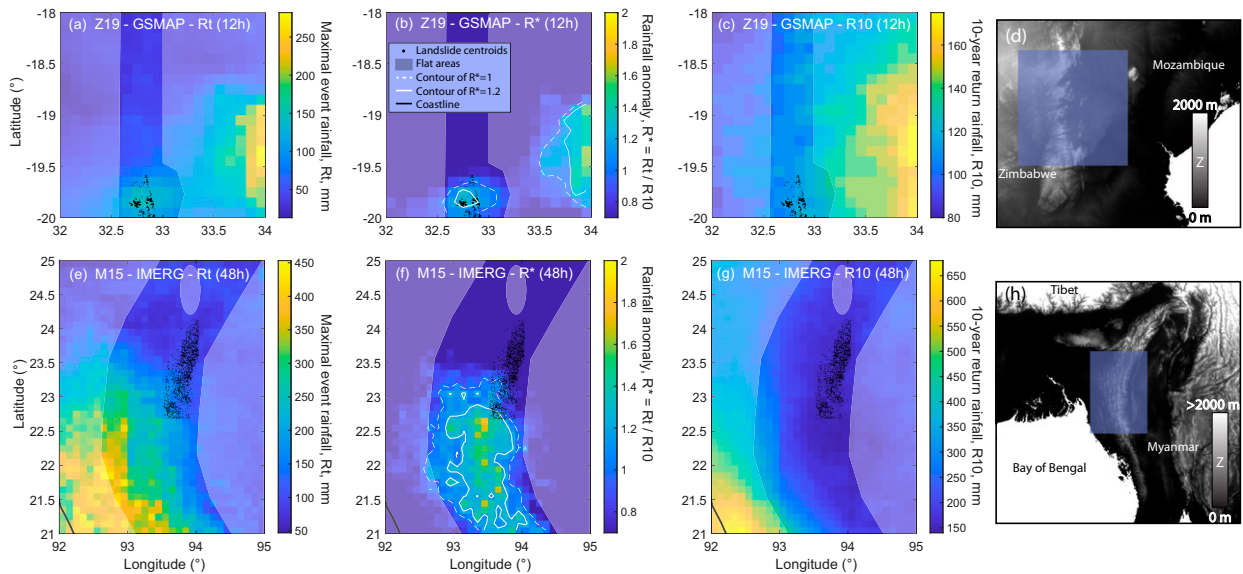
FIG. 1. (left) Maximal total rainfall ( R_t ; mm), (left center) rainfall anomaly ( R^* = R_t/R_{10} ), and (right center) 10-yr return rainfall ( R_{10} ; mm) obtained (a)–(c) from GSMaP at 12-h time scale during Z19 and (e)–(g) from IMERG at the 48-h time scale during M15. Also shown for context are (d), (h) elevation maps of the respective regions containing the study area (in blue). Black dots are landslide centroids, shaded areas are relatively flat terrain where landsliding is unlikely, and white solid and dashed lines in (b) and (e) are the anomaly contour for R^* = 1.2 and 1, respectively. Note that the sharp, linear boundaries of the landslide inventory in (e)–(g) are defined by the footprint of the two Sentinel-2 images that were used for the mapping and that there is evidence of some landsliding occurring beyond these boundaries (see the online supplemental material). Note how the difference in patterns between R_t and R^* is related to the existence of strong spatial gradients in R_{10} .
