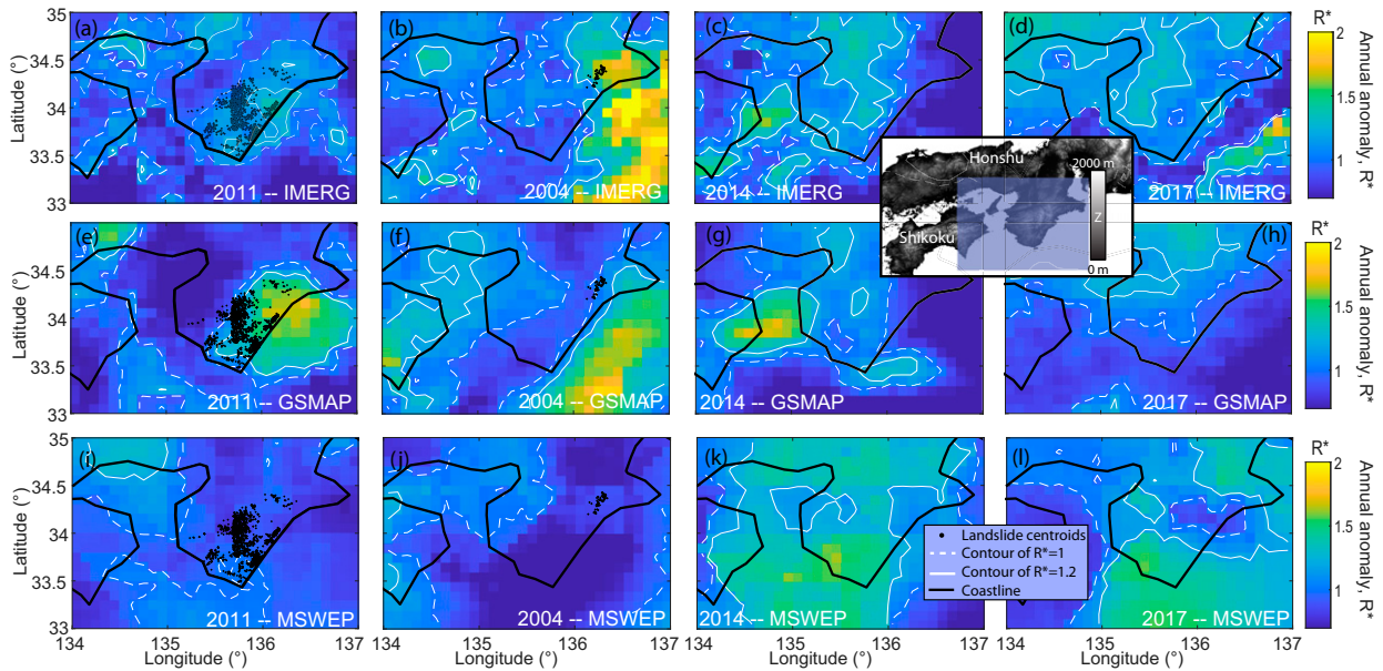
FIG. 2. Maps of the maximal annual anomalies at 48 h, for four selected years over the Kii Peninsula (Japan), for (a)–(d) IMERG, (e)–(h) GSMaP, and (i)–(l) MSWEP. Black dots show landslide centroids from two major landslide events that occurred during Typhoons Meari in 2004 [in (b), (f), and (j)] and Talas in 2011 [in (a), (e), and (i)]. The timing of these maxima is in Fig. S14 in the online supplemental material. For context, an elevation map of the region containing the study area (in blue) is shown in the inset. Note the difference between products in terms of anomaly retrieval during landslide events in 2011 and 2004, as well as the retrieval large anomalies in 2014 and 2017, although no landslide events were reported.
