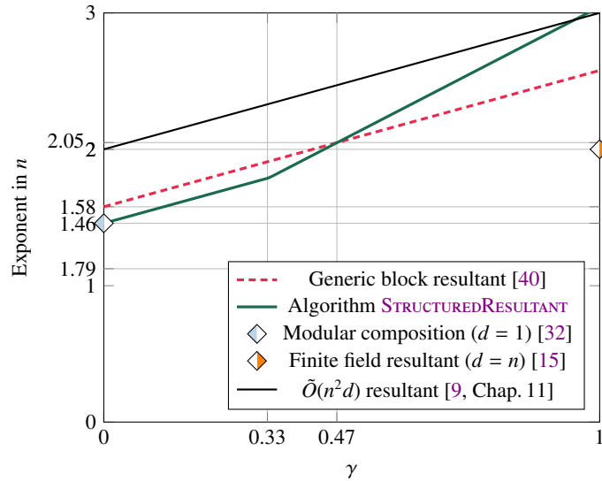
Figure 1. Comparison of known asymptotic cost bounds for the resultant of generic polynomials. Exponents in n with d = n^\gamma and \omega = 2.373 .
