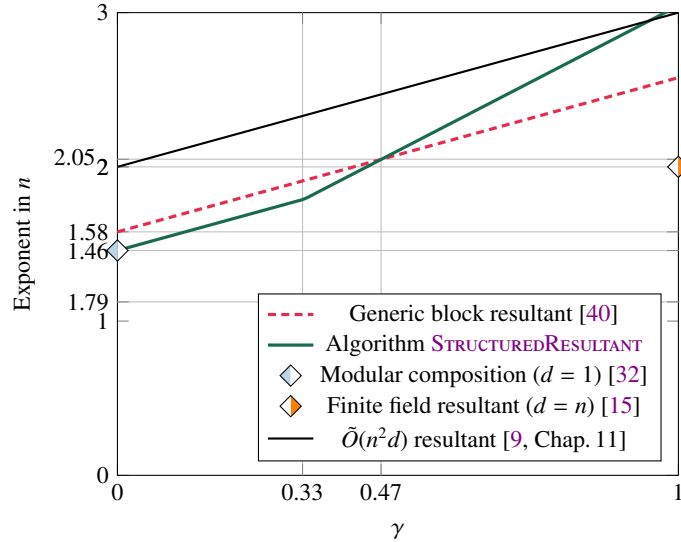
Figure 1. Comparison of known asymptotic cost bounds for the resultant of generic polynomials. Exponents in n with d = n^\gamma and \omega = 2.373 .
