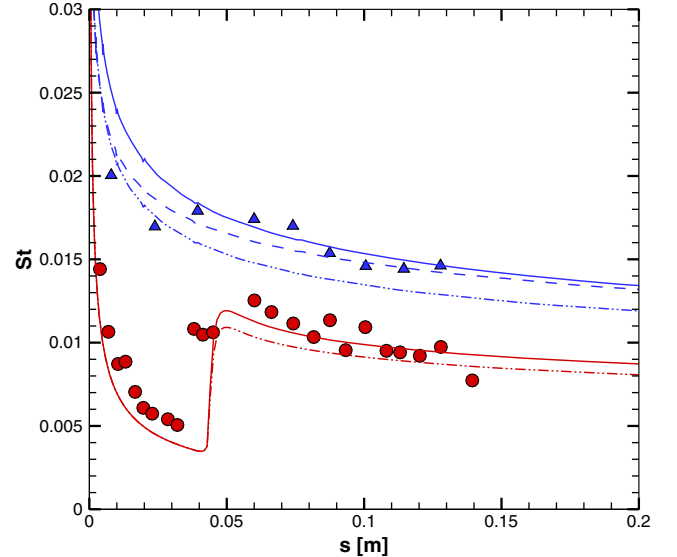
Fig. 2 Stanton number St distributions for smooth and rough cases of biconic configuration at Mach 11: smooth wall (circles), and rough wall (triangles). Full lines are results obtained using k - \omega SST model without compressibility corrections (solid), with Zeman correction (dashed), with Sarkar correction (dashed-dotted-dotted).
