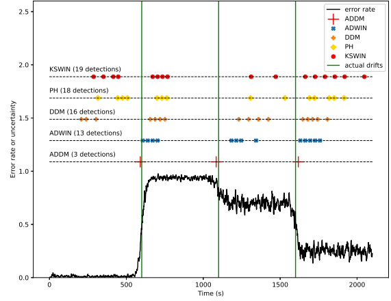
Fig. 2. Detected drifts on the Mixed data set. The vertical lines in green are the actual drifts points. The horizontal lines show the detected drifts by each detector. The horizontal line with red plus (+) markers shows our method’s detections.
