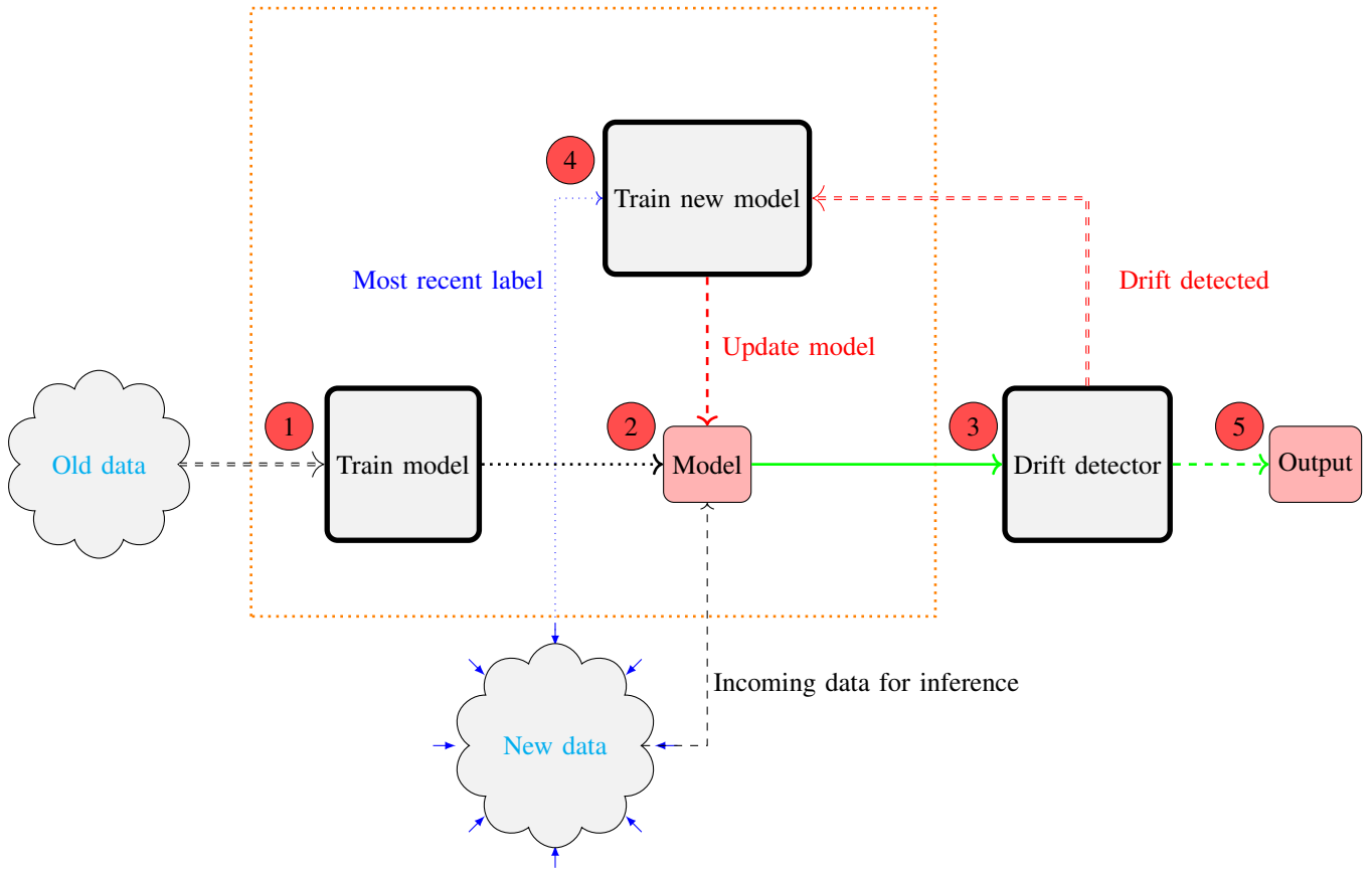
Fig. 1. Architecture and Dataflow of ADDM. ① Train a predictive model with old data set. ② Predict new incoming data and compute the error rate. ③ Search for changes in the model’s error rate. If drift is detected, triggers a signal to update the model. ④ Train new model with most recent data if drift is detected and update the old model. ⑤ Predict the final output with updated model.
