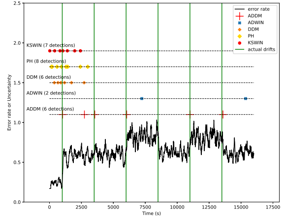
Fig. 3. Detected drifts on the Brieman 2d planes data set. The vertical lines in green are the actual drifts points. The horizontal lines show the detected drifts by each detector. The horizontal line with red plus (+) markers shows our method’s detections.
