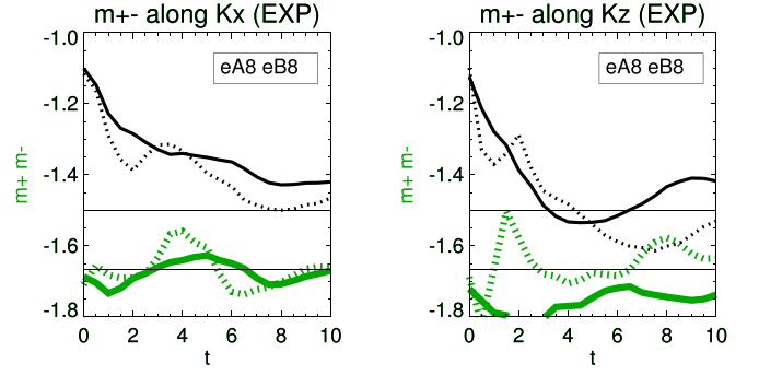
Figure 14. Spectral indices m_+ (solid lines) and m_- (dotted lines) vs. time computed in the radial ( 4 \leq k_x \leq 10 ; left panel) and z ( 4 \leq k_z \leq 10 ; right panel) directions. Shown are runs eA8 (thick green lines) and eB8 (thin black lines).
