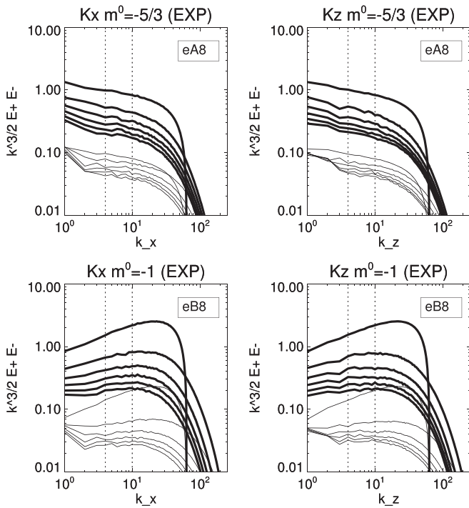
Figure 13. The E_+ (thick lines) and E_- (thin lines) spectra along the radial ( k_x ; left panels) and perpendicular ( k_z ; right panels) directions for two runs with expansion: eA8 (top) and eB8 (bottom). Times t = 0, 2, \dots, 10 , spectra are compensated by k^{-3/2} . Dotted lines are the boundaries of the interval used to compute the spectral indices.
