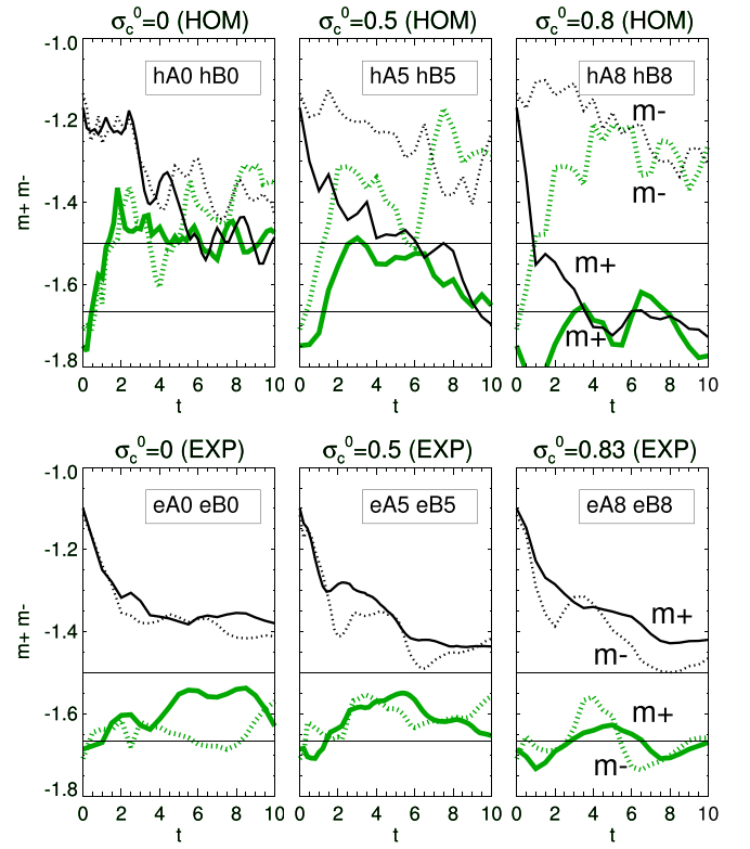
Figure 8. Varying \sigma_c^0 and m_0 . Shown are indices m_+ and m_- vs. time (solid and dotted lines, respectively) computed in the normalized wavenumber interval 4 \leq k \leq 10 . Each panel shows two runs with a given \sigma_c^0 (from left to right, 0, 0.5, 0.8, 0, 0.5, and 0.83). Runs with m_0 = -5/3 appear as double thick green lines, and runs with m_0 = -1 appear as thick black lines. Solid horizontal lines mark spectral indices -3/2 and -5/3 .
