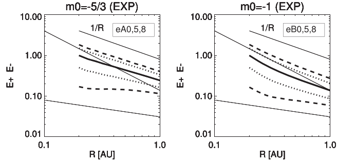
Figure 4. Varying cross helicity: total energies E_{\pm} vs. heliocentric distance R for runs with expansion eAs and eBs . Styles are the same as in Figure 3. The two long thin solid lines are the mean energies E_+ and E_- as found by Bavassano et al. (2000, 2002) from Helios data, and the short thin solid line is the 1/R (WKB) decay.
