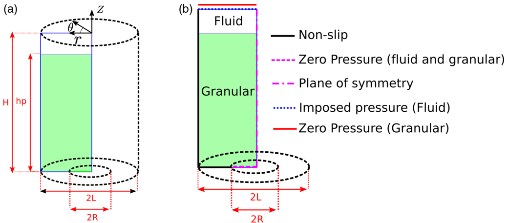
FIG. 11. (a) Configuration and (b) boundary conditions of the continuum simulation for the discharge of a silo with a pressurized gas at its top in a cylindrical geometry.
