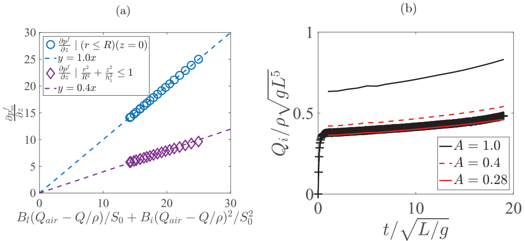
FIG. 13. (a) Average pressure gradients of the fluid phase on the outlet section ( \circ ) and on an ellipsoidal zone above the outlet ( \diamond ) as a function of B_1(Q_{\text{air}} - Q/\rho)/S_0 + B_2(Q_{\text{air}} - Q/\rho)^2/S_0^2 . (b) Temporal evolution of the nondimensional discharge flow rate of the granular media Q/\rho\sqrt{gL^5} for R = 0.25L and p_{\text{air}} = 5\rho gL and comparison with the prediction of the model with different coefficient values \mathcal{A} .
