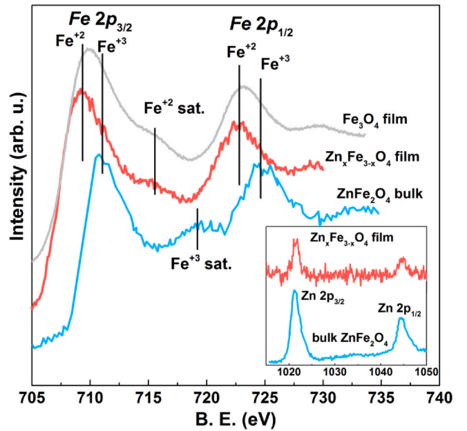
Fig. 3. Fe 2p spectra for Zn_xFe_{3-x}O_{4-\delta} and Fe_3O_4 thin films at T_C = 500 °C. Inset shows Zn 2p spectra of corresponding samples. For comparison, Fe 2p and Zn 2p spectra of bulk ZnFe_2O_4 are also included.
