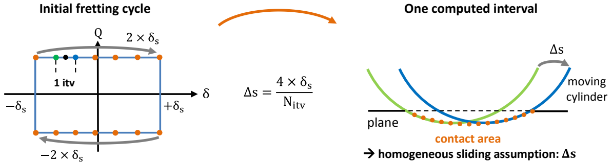
Fig. 2. Description of the incremental description of the sliding contact: after each \Delta s sliding increment expressed as a function of the sliding amplitude \delta_s and the number of iterations during the alternated sliding cycle ( N_{itv} ), the WK contact algorithm is applied to extract the corresponding pressure profile and the related increment friction of friction energy density.
