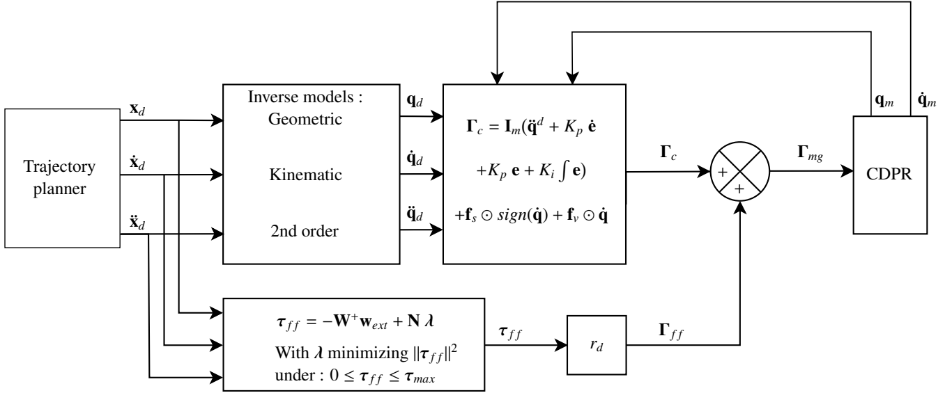
Figure 13: Control scheme of the CDRP with the pseudo-inverse tension distribution
