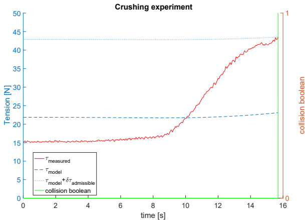
(b) Evolution of the tensions in the cable 1 during a circular translation with a prolonged collision, i.e. a crushing situation.
