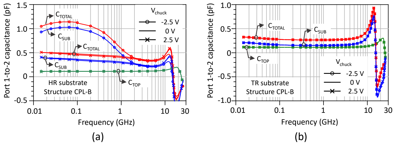
Figure 6. Coupling capacitances between the electrode combs of structure CPL-B at chuck bias of -2.5, 0 and 2.5 V. C_{TOTAL} is the total measured capacitance, C_{TOP} is the capacitance mainly associated with the interconnects, C_{SUB} represents the contribution of the substrate to the lateral capacitive coupling. (a) HR starting substrate; (b) TR starting substrate.
