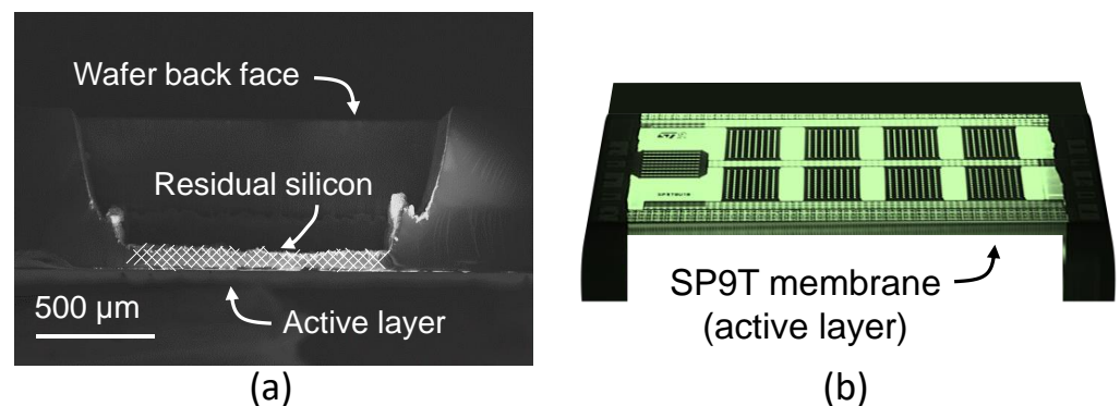
Figure 9. (a) SEM cross-sectional image of cavity fabricated using laser processing. The hatched zone corresponds to residual silicon left after laser processing and before XeF 2 selective etching; (b) 3D rendered backlight illuminated optical microscope image.
