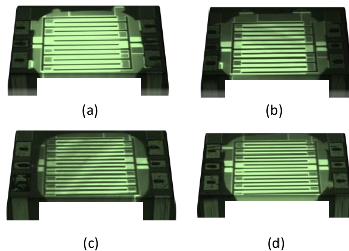
Figure 3. DLM images of capacitive coupling structures suspended in a membrane after substrate removal: (a) CPL-A/HR-SOI; (b) CPL-A/TR-SOI; (c) CPL-B/HR-SOI; (d) CPL-B/TR-SOI.
