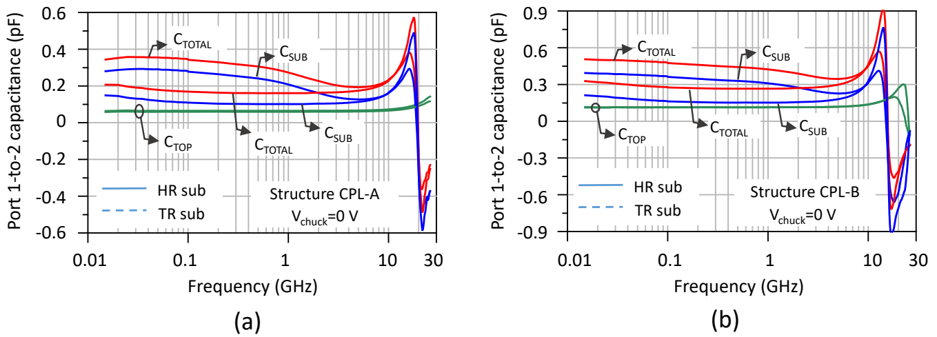
Figure 5. Coupling capacitance between the electrode combs. C_{TOTAL} is the total measured capacitance, C_{TOP} is the capacitance mainly associated with the interconnects, C_{SUB} represents the contribution of the substrate to the lateral capacitive coupling. (a) Structure CPL-A; (b) structure CPL-B.
