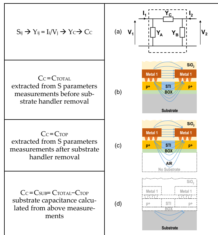
Figure 4. Extraction of capacitive coupling between interdigitated electrode combs. (a) Principle of extraction of coupling admittance Y C from the measured admittance matrix Y ij ; (b) extraction of coupling capacitance C TOT ; (c) extraction of capacitance C TOP after local substrate removal; (d) deduction of the substrate coupling capacitance.
