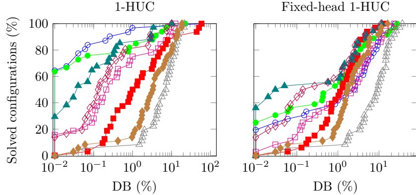
Figure 8: Proportion of configurations solved with their VBS where the DB is under a DB threshold
