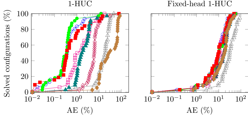
Figure 7: Proportion of configurations solved with their VBS where the AE is under an AE threshold
