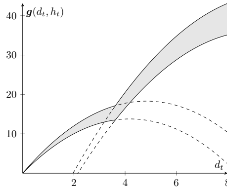
Figure 3: Function \mathbf{g} with polynomial functions
