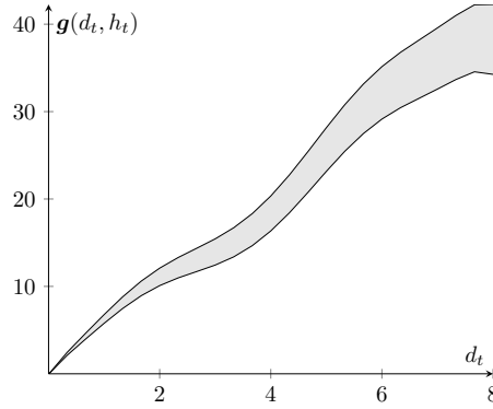
Figure 5: Function \mathbf{g} with a single polynomial function
