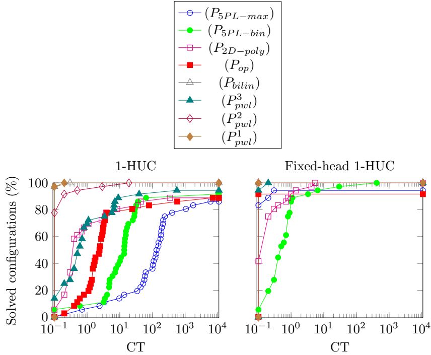
Figure 6: Proportion of configurations solved with their VBS where the CT is under a CT threshold
