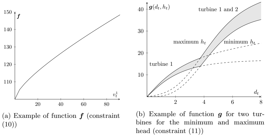
Figure 2: Examples of function f and g
