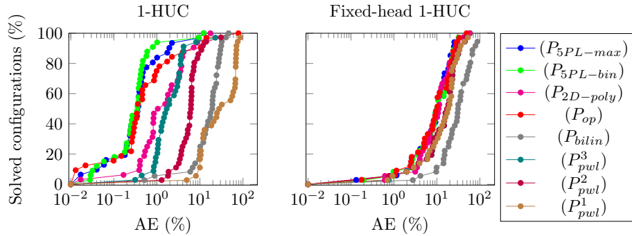
Figure 8: Proportion of configurations solved with their VBS where the AE is under an AE threshold
