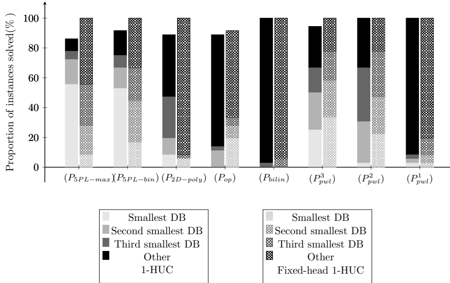
Figure 10: Proportion of configurations for each model solved by their VBS
