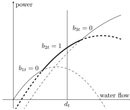
Figure 4: Polynomial functions representing the power for each combinations of turbines
