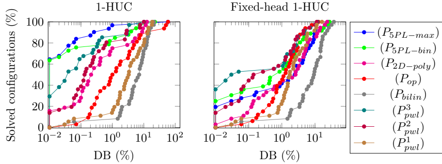
Figure 9: Proportion of configurations solved with their VBS where the DB is under a DB threshold
