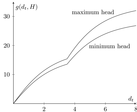
Figure 3: Example of function g for the minimum and maximum head (constraint (4))
