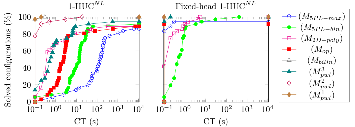
Figure 10: Proportion of configurations solved with their VBS where the CT is under a CT threshold
