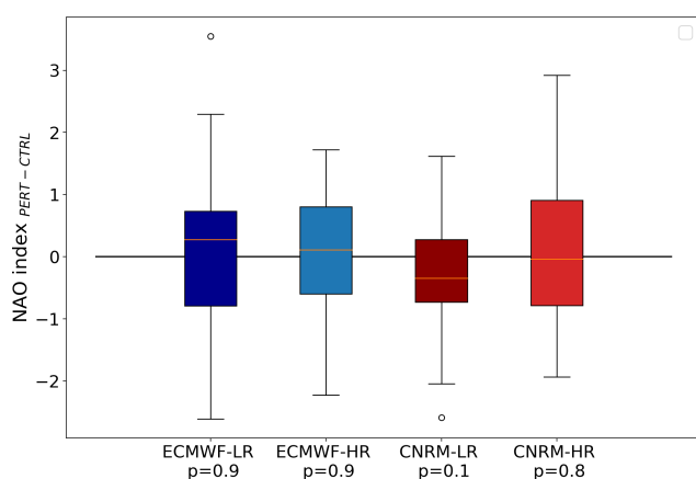
Figure A3. Boxplot of the summer NAO index (station-based method) in PERT compared to CTRL, where the CTRL has been taken as the 40-year reference period, for all members in each model. The p value of a Kolmogorov–Smirnov test between PERT and CTRL is shown below each boxplot.
