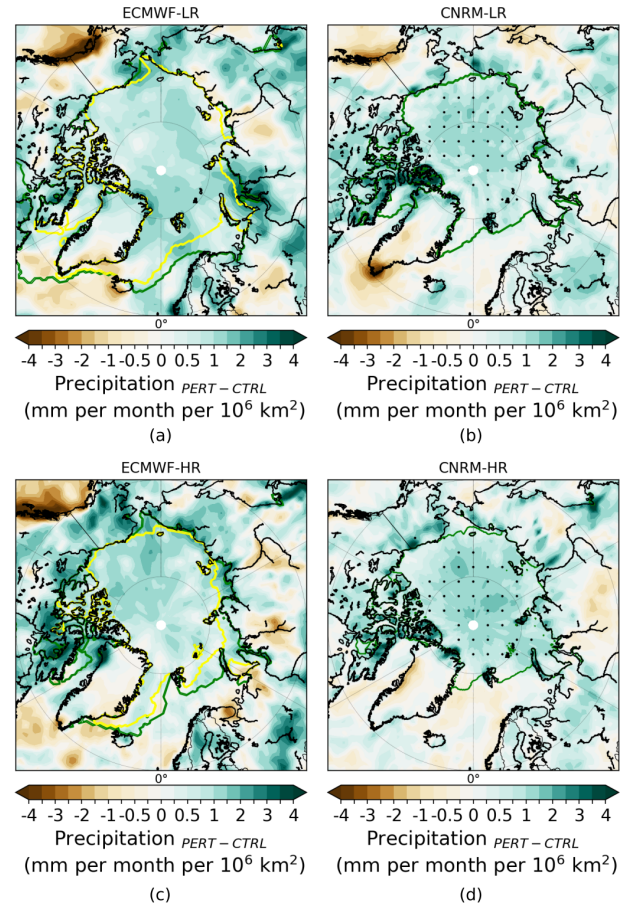
Figure 9. Ensemble mean changes ( PERT-CTRL ) in summer (JAS) precipitation scaled by the amount of sea ice extent loss for ECMWF-LR (a), CNRM-LR (b), ECMWF-HR (c) and CNRM-HR (d). The dots show where the response is statistically significant according to a 10 % level FDR test associated with a Kolmogorov–Smirnov test. The green and yellow lines represent the sea ice edge (15 % ice concentration) from CTRL and PERT, respectively.
