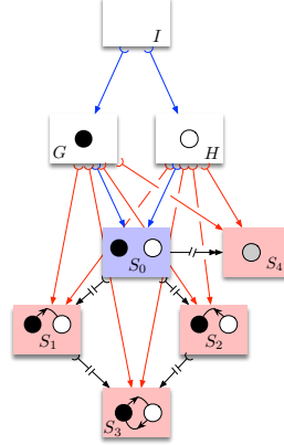
Figure 4: Example for an \mathcal{M} -multi-sum \Sigma_{\mathcal{M}}(\bullet, \bullet) of one-vertex graphs in SGraph (i.e., for \mathcal{M} = \text{rm}(\text{SGraph}) ). Note in particular the monic-epis that extend the two-vertex graph S_0 into the graphs S_1, S_2 and S_3 , all of which have the same vertices as S_0 (recalling that a morphism in SGraph is monic/epic if it is so on vertices), yet additional edges, so that in particular none of the morphisms S_0 \rightarrow S_j for j = 1, 2, 3 is edge-reflecting.
