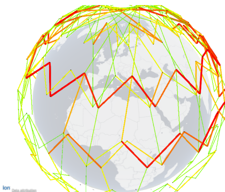
Fig. 9: Example of flow distribution around Earth with UMCF routing algorithm and 4 Mbps ISL. Red links show congestion.
