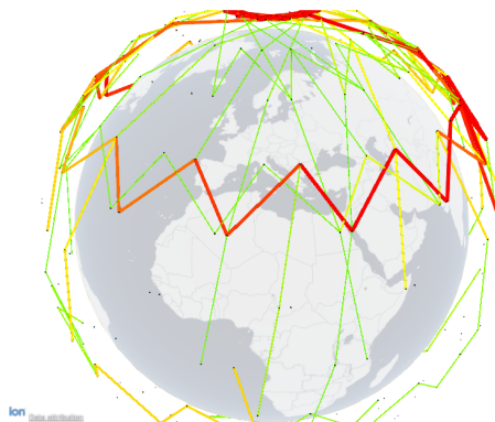
Fig. 8: Example of flow distribution around Earth with Shortest Path routing algorithm and 4 Mbps ISL. Red links show congestion.
