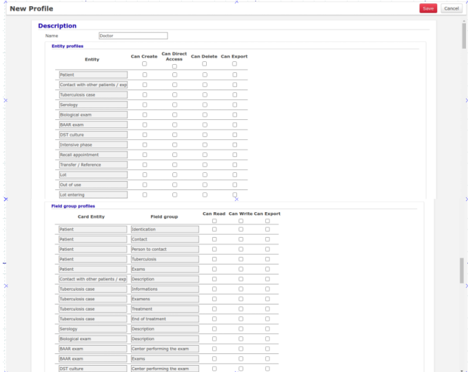
Figure 9: Interface presenting how rights are assigned to users
