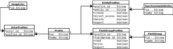
Figure 8: The class diagram of users management in the EPICAM platform
