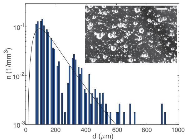
Figure A.14: Histogram of the bubbles diameters obtained by image analysis. Here for sample D at 500 rpm. Result of the fitting with a lognormal law is shown by the black line. We obtain R_0 = 85 \mu\text{m} , \epsilon = 0.65 and \Phi = 1.8\% . Inset: a typical image. The bar is 2 mm long.
