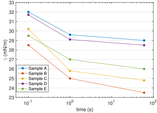
Figure 1: Surface tension as a function of time for the five samples.
