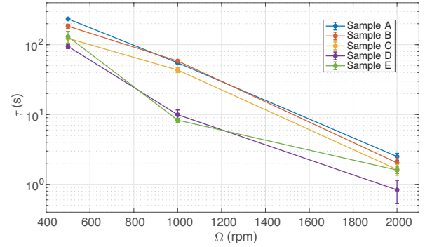
Figure 7: Time for reaching a steady state ( \tau ) as a function of the speed of rotation ( \Omega ) for the five oils. We see that formulations D and E aerated faster than the other oils.
