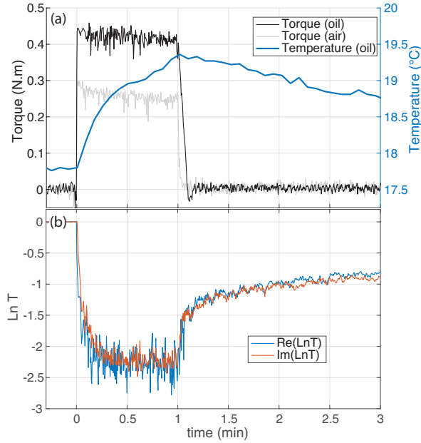
Figure 3: Illustrations of the data acquired during a run, here for 1 minute of rotation at \Omega = 2000 rpm in oil A. (a) Torque and temperature as functions of time. (b) Logarithm of the ultrasonic complex transmission at 5 MHz.
