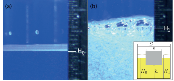
Figure 4: Examples of images acquired before (a) and just after (b) the rotation of the gear, in oil A at \Omega = 2000 rpm. The initial height of oil H_0 is increased to H_1 because of the air entrained. The inset shows the geometrical parameters needed for calculating the air volume fraction from this change of oil level (eq. 1). Here we find H_0 = 8.02 cm and H_1 between 8.42 and 8.58 cm, leading to \Phi_{\text{opt}} = 3.3 \pm 0.5\% .
