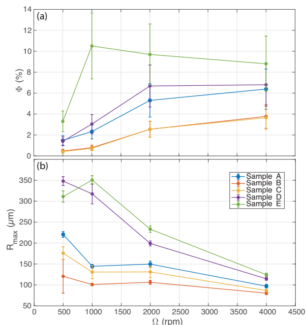
Figure 8: \Phi (top) and R_{\max} (bottom) as functions of \Omega for the five oils, in the steady state of turbulent mixing. There is a clear effect of the formulation: B and C tend to entrain less air, with small bubbles, while D and E have larger bubbles and more air.
