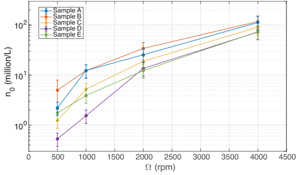
Figure 12: Number of bubbles per unit volume, n_0 (in million per liter), as a function of \Omega , for the different samples.
