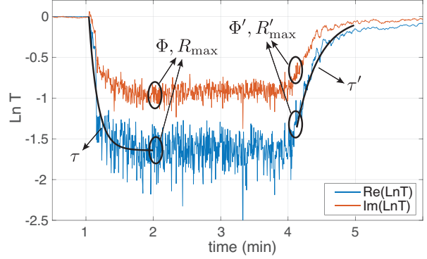
Figure 6: Illustration of the 6 parameters extracted from the ultrasonic measurements, here for sample E at 1000 rpm. \Phi , R_{\max} and \tau provide information on the aeration phase, while \Phi' , R'_{\max} and \tau' are used to characterize the deaeration phase.
