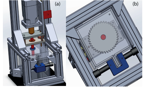
Figure 2: 3D drawings of the setup. General (a) and bottom (b) views. The ultrasonic extension is clearly visible on the bottom view. It consists of two transducers (dark grey cylinders) held by a clip (in blue) on the 5 mm-wide chamber of the casing, allowing for the measurement of the ultrasonic transmission through the aerated oil.
