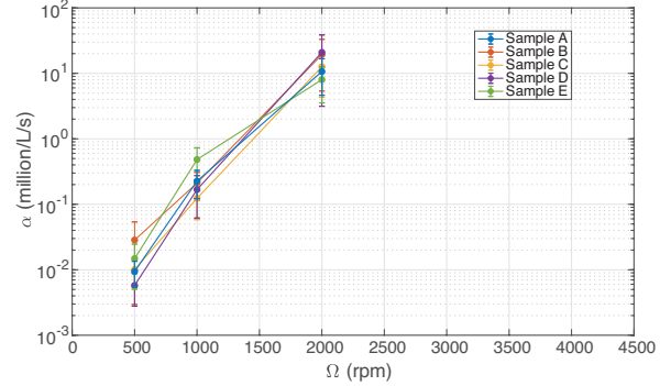
Figure 13: Rate of bubble production, \alpha , as a function of \Omega , for the different samples.
