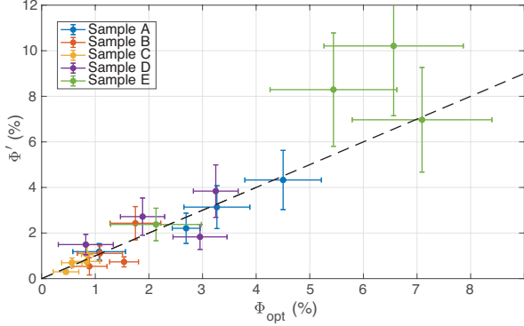
Figure 10: Aeration when the motor stops as measured acoustically ( \Phi' ) and optically ( \Phi_{\text{opt}} ). The agreement is reasonable, which suggests that the bubbles visiting the 5 mm extension are well representative of the total population of bubbles.
