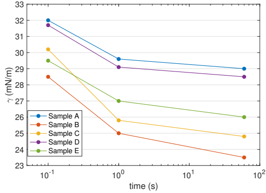
Figure 1: Surface tension as a function of time for the five samples.
