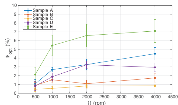
Figure 9: Volume fraction of air as a function of \Omega as given by the analysis of the images taken within 2 seconds after the motor has stopped. The levels of aeration are smaller than in the mixing phase (see Fig. 8a).
