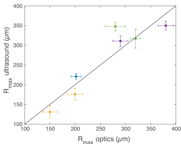
Figure A.15: Comparison of values of R_{\text{max}} obtained by the ultrasonic analysis (y-axis) and the optical one (x-axis), for oil A at 500 rpm (blue symbol) and samples C, D, E at 500 and 1000 rpm.
