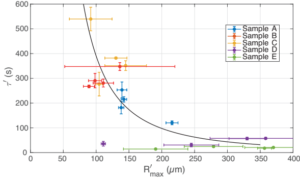
Figure 11: Deaeration time \tau' as a function of R'_{\text{max}} , the radius of the larger bubbles in the oil, when the motor stops. We find that the larger the bubbles the quicker the deaeration process. The solid line is a guide for the eyes (not a fit) of a 1/x^2 law.
