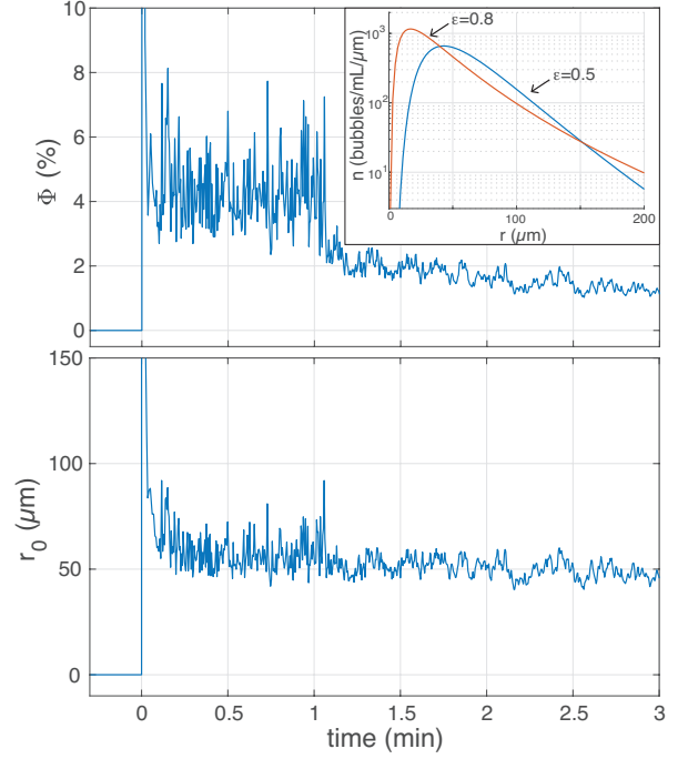
Figure 5: Air volume fraction ( \Phi ) and bubble median radius ( r_0 ) obtained by analyzing the ultrasonic data from Fig. 3b, assuming that the polydispersity is 0.5. The inset shows the distributions one obtains one minute after the start of the motor, when assuming a polydispersity of 0.5 (blue) or 0.8 (red).
