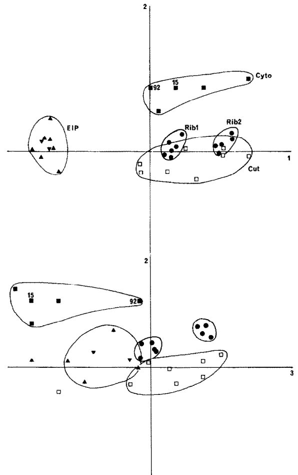
Fig.2. Multivariate analysis of the proteins contained in the data base. The planes constituted by the 1–2 (top) and 2–3 (bottom) axes are represented. Group 1 (cuticle), □; group 2 (cytoskeleton), ■; group 3a and b (ribosome), ● and group 4 (EIP), ▲.
