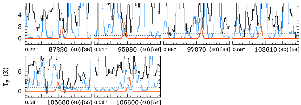
Fig. B.5. Same as Fig. B.3, but for transitions of vinylamine C 2 H 3 NH 2 between the tunneling states 0 - and 0 + .
