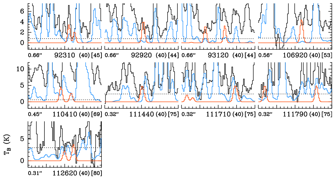
Fig. B.4. Same as Fig. B.3, but for transitions of vinylamine C 2 H 3 NH 2 within the tunneling states 0 + and 0 - .
