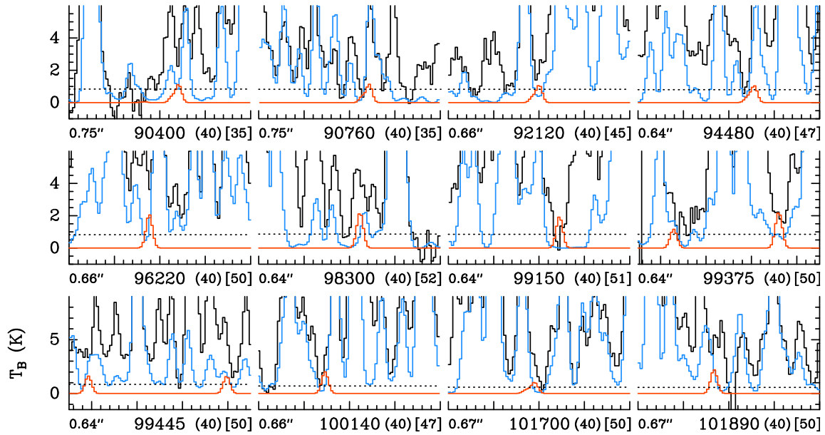
Fig. B.3. Same as Fig. B.1, but the red spectrum shows the synthetic spectrum of ethanamine anti -C 2 H 5 NH 2 , v =0 used to derive the upper limit on its column density reported in Table 6. The blue spectrum does not contain the contribution of the species shown in red.
