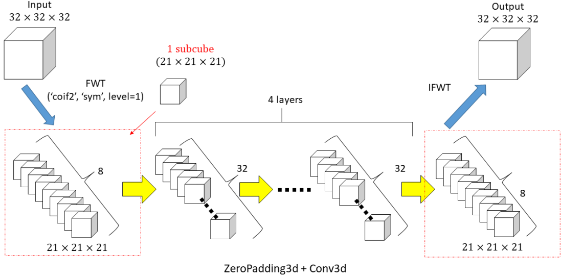
Figure 1: Illustration of SR network structure.
