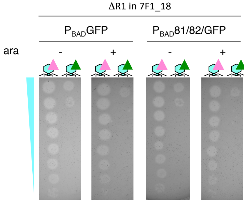
Figure S10 The two pink phage specific genes are not involved in R-M III neutralization. The two genes (p0081 and 82 in phage 431E46.1) were cloned between the pBAD promoter and the gfp gene, leading to a transcriptional fusion ( P_{BAD}81/82/GFP ). A plasmid expressing only the gfp gene ( P_{BAD}GFP ) was used as control. These plasmids were transferred by conjugation into the 7F1_18 derivative \Delta R1 , lacking the R1 region but carrying the R2 region, thus the R-M III system. Gene expression was induced (+) or not (-) with 0.2% arabinose (as visualized by fluorescence microscopy of the GFP). Tenfold dilutions of pink (431E42.2) and green (234P8) phages were spotted on the \Delta R1 strain derivatives. Experiment was performed twice and images are representative of two independent experiments.
