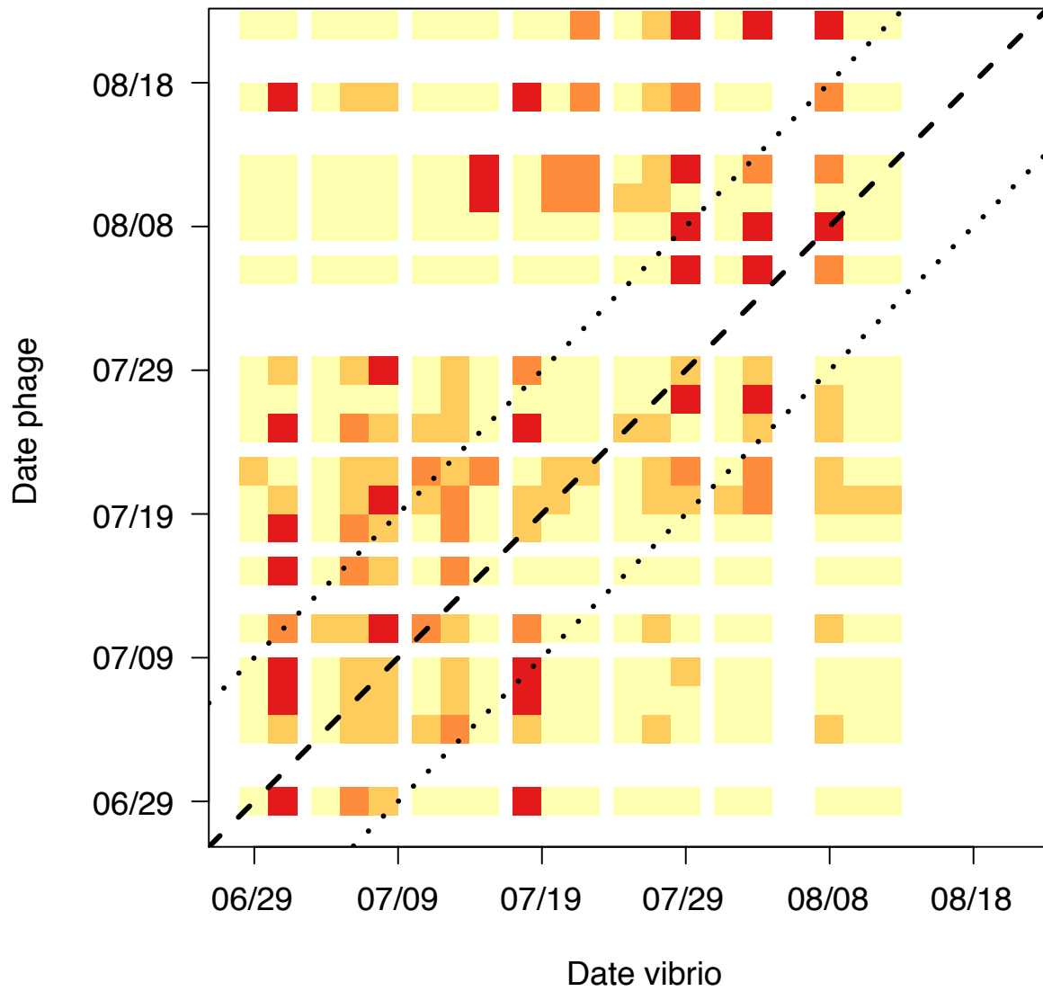
Figure S6. Temporal pattern of adaptation at small time scales obtained from the intensive sampling carried out in Brest. The mean infectivity is a function of the date of V. crassostreae and date of phages in cross-inoculation experiments. Yellow: mean infectivity 0%, light orange: mean infectivity in 0-10%, dark orange: mean infectivity in 10-20%, red: mean infectivity greater than 20%. The diagonal (dashed line) shows the contemporaneous combinations, the sub-diagonals (dotted lines) the combinations shifted by \pm 10 days.
