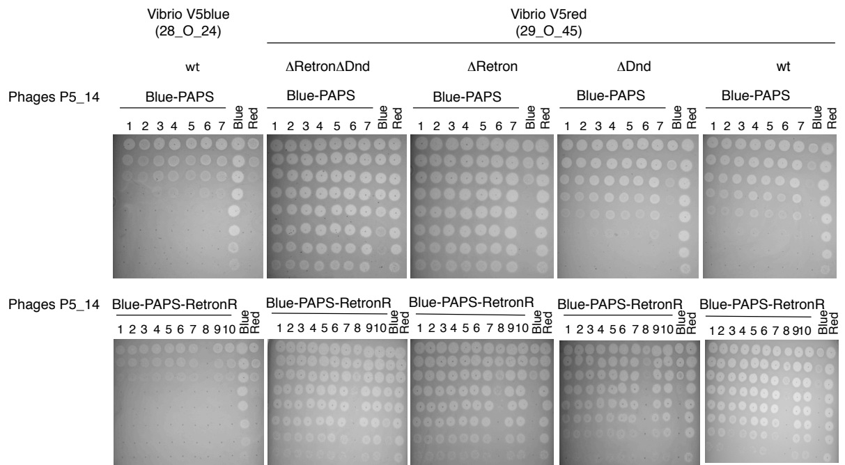
Figure S11. Changes in susceptibility to phage killing observed for phage-defence region deletions in one strain (29_O_45) of vibrio clade V5. Lawns of bacterial hosts with drop spots of a 1:10 dilution series of phages P5_14 blue (66E30.1), red (44E38.1) and several isolates of blue phage mutants (Blue-PAPS and Blue-PAPS-RetronR). Experiment was performed twice and images are representative of two independent experiments.
