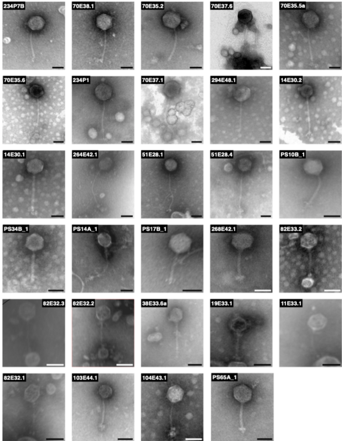
Figure S4. Transmission electron micrographs of 29 siphoviruses. Scale bars represent 50nm.
