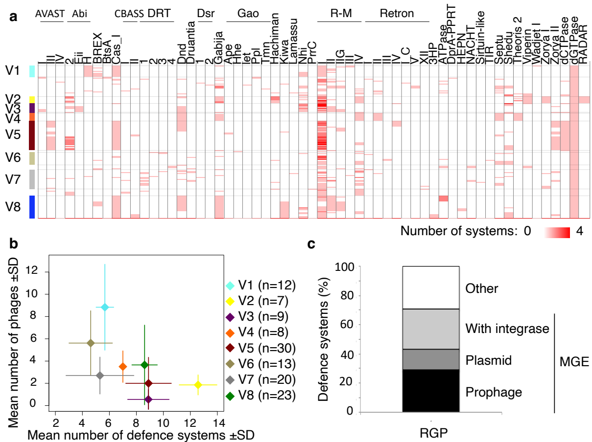
Figure 4. Distribution of phage-defence systems in V. crassostreae genomes.
