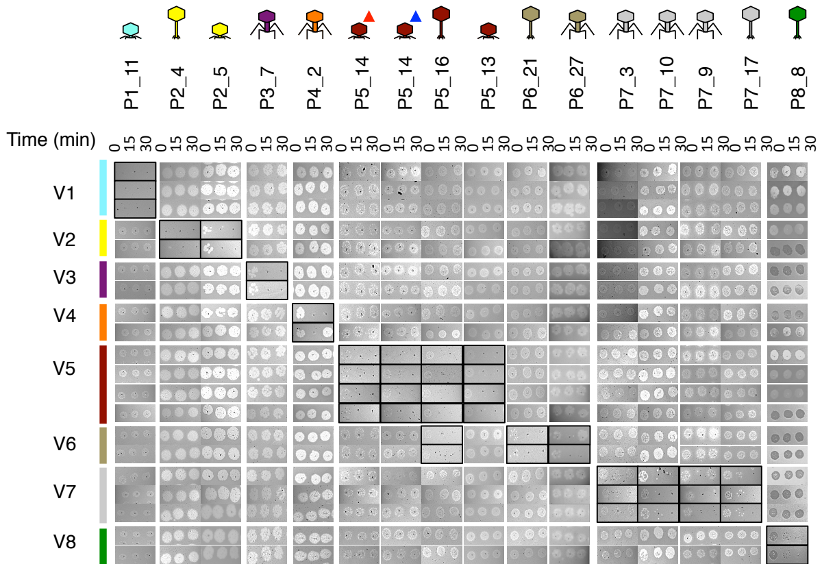
Figure S5. Phage adsorption estimation using representatives of the vibrio clades and phage clusters. After allowing a concentration of phages (MOI 0.01) to adsorb to a V. crassostreae strain for 15 and 30 minutes, free phages that remained unattached were serially diluted and plated with sensitive hosts to quantify adsorption. Bacteria and phage belonging to a specific clade and cluster are arrayed in rows and columns, respectively. We highlight two phages (indicated by red and blue triangles) from phage cluster P5_14 differing in their host range (blue and red in the main text). Combinations of phage and host leading to a drop in the number of phages in the supernatant (indicating an adsorption) are surrounded by bold frames. Images are representative of two independent experiments.
