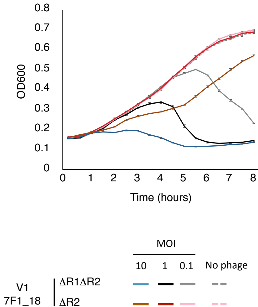
Figure S8. The region R1 that is specific to the strain 7F1_18 from V1 clade and is involved in phage resistance does not seem to act via an abortive infection mechanism. Within region R1, two genes, encoding a putative NTPase (GV2333_v1_250051) and an adenosine deaminase (GV2333_v1_250052) are involved in the defence against the P1_12 siphoviruses. Because a two-gene cassette named RADAR, consisting of an adenosine triphosphatase and a divergent adenosine deaminase, was previously demonstrated to cause abortive infection, we explored whether the R1 region confers a similar phenotype. We compared the P1_12 phage (70E37.6) infection dynamics of 7F1_18 lacking only R2 ( \Delta R2 ) or both the R1 and R2 ( \Delta R1\Delta R2 ). At a MOI of 0.1, 1 and 10, \Delta R1\Delta R2 cell cultures collapsed owing to phage propagation after 5.5, 4 and 1 hours, respectively. \Delta R2 cultures were viable, growing similarly to the control (no phage) at a MOI of 0.1 and 1, while at MOI of 10 the culture did not reach a state of growth stasis although we observed a delayed growth. Therefore, these results do not allow us to demonstrate a function of region R1 in abortive infection. Infections were performed in technical triplicate ( \pm SD from three replicates). Data are representative of two independent experiments.
