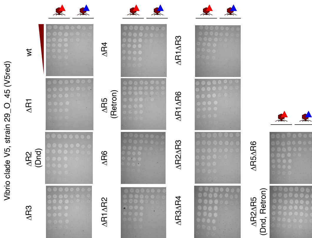
Extended Data Figure 6. Changes in susceptibility to phage killing observed for V5red specific region deletions. Single and double deletions of the six regions found in all V5red and absent in all V5blue strains were performed in one strain (29_O_45) of vibrio clade V5. Lawns of bacterial hosts with drop spots of a 1:10 dilution series of phages from cluster P5_14, red (red triangle; phage) and blue (blue triangle). The red phages were 36E38.1, 41E34.2, 44E38.1 and 44E38.2. The blue phages were 24E30.2, 24E35.2, 64E30.1 and 66E30.1.
