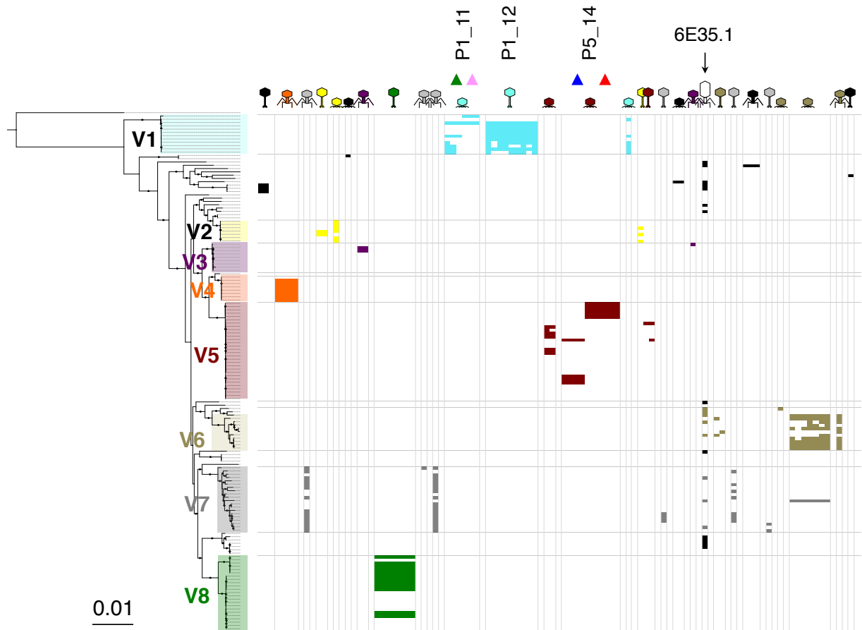
Figure 1. A modular phage-vibrio infection network.
