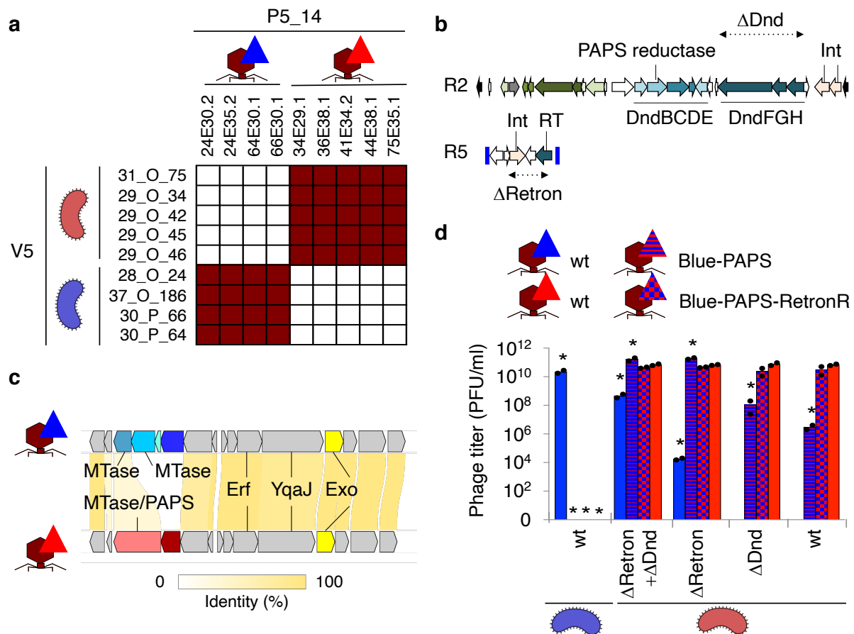
Figure 6. Bacterial defence and phage counter-defence.
