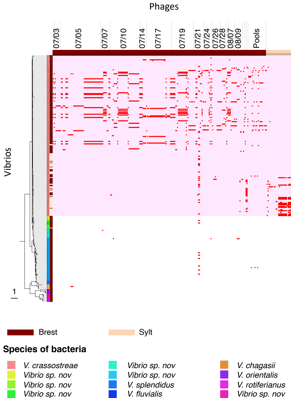
Extended Data Figure 2. Host range matrix for assay of phages on gyrB -sequenced hosts. Rows represent vibrio strains (n=299), columns represent phages (n=243 phages isolated in Brest and ordered by date or “Pools” when phages were isolated from a mix of viruses from 5 consecutive dates; n=31 phages isolated in Sylt), red marks indicate infection of host. Pink shade discriminate V. crassostreae isolates from representatives of other species.
