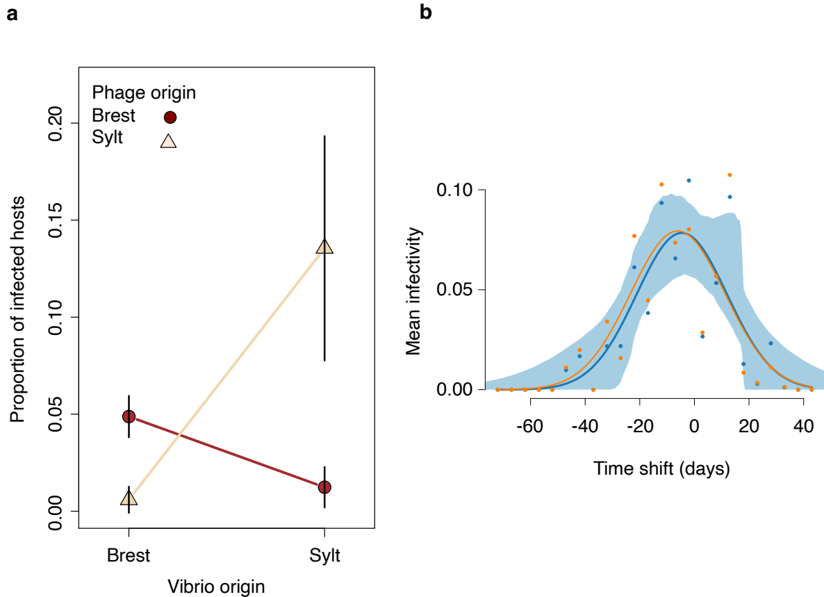
Figure 3. Patterns of phage adaptation across space and time.
