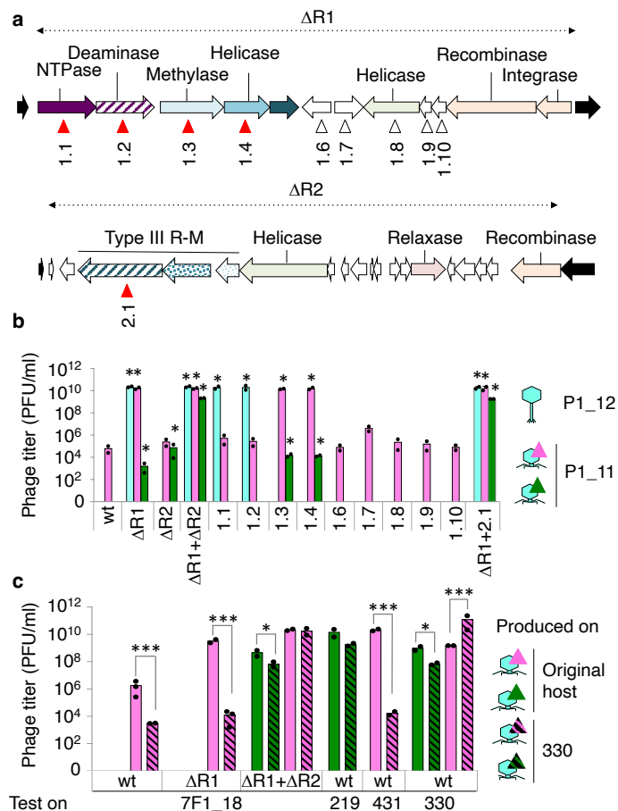
Figure 5. Anti-phage systems identified in V. crassostreae clade V1.
