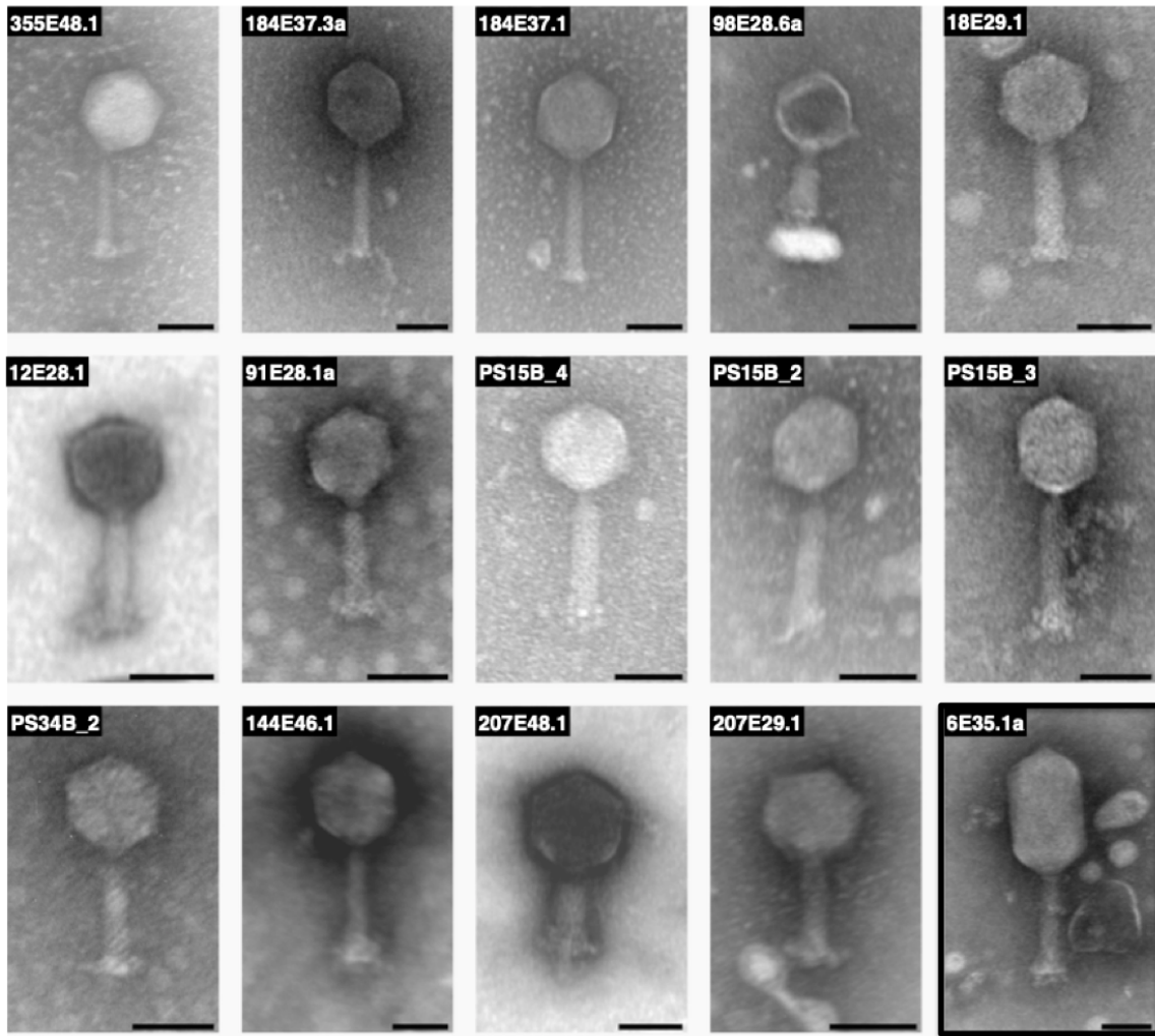
Figure S3. Transmission electron micrographs of 15 myoviruses. The broader host range phage 6E35.1a is surrounded in bold. Scale bars represent 50nm.
