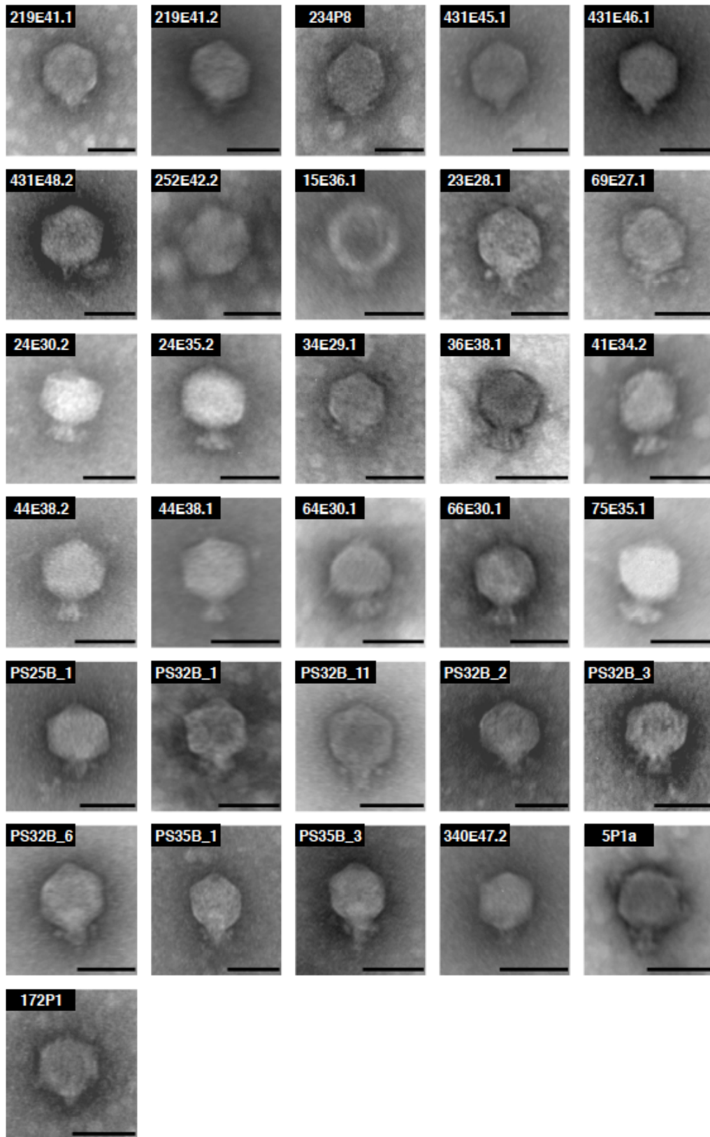
Figure S2. Transmission electron micrographs of 31 podoviruses. Scale bars represent 50nm.
