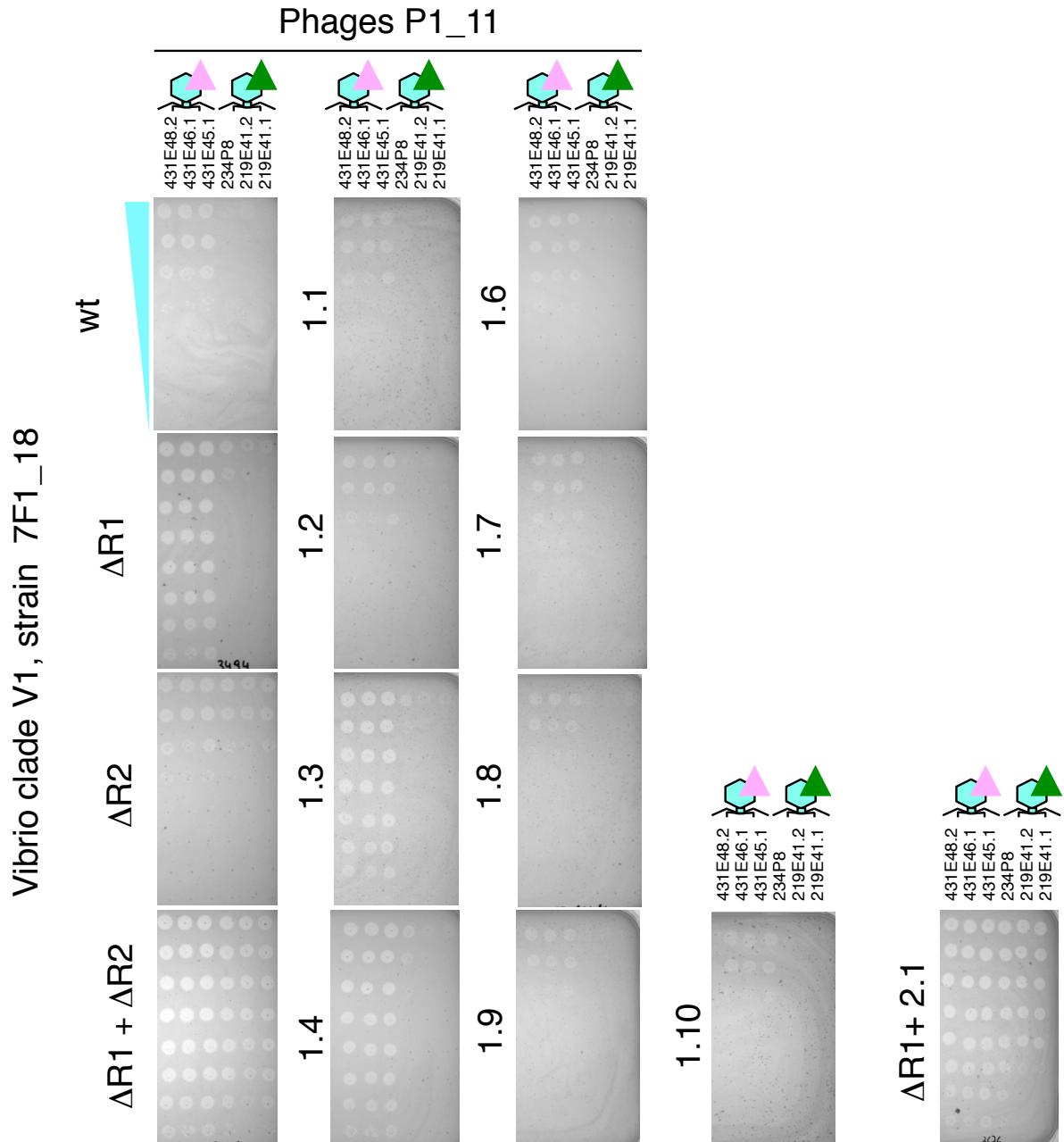
Figure S9. Changes in susceptibility to phage killing observed for phage-defence region deletions or gene inactivation in one strain (7F1_18) of vibrio clade V1. Tenfold dilutions of phages from cluster P1_11 were spotted on the strain 7F1_18 wild type and derivatives ( \Delta R1 , \Delta R2 for complete deletion of strain specific region R1 and R2; 1.1 to 1.10 for gene inactivation in R1, 2.1 for gene inactivation in R2, after integration of a suicide vector. Based on their infectivity the P1_11 phages were distinguished into those being produced (pink triangle) and not being produced (green triangle) by the strain 7F1_18 from clade V1. All experiments were performed twice and images are representative of two independent experiments.
