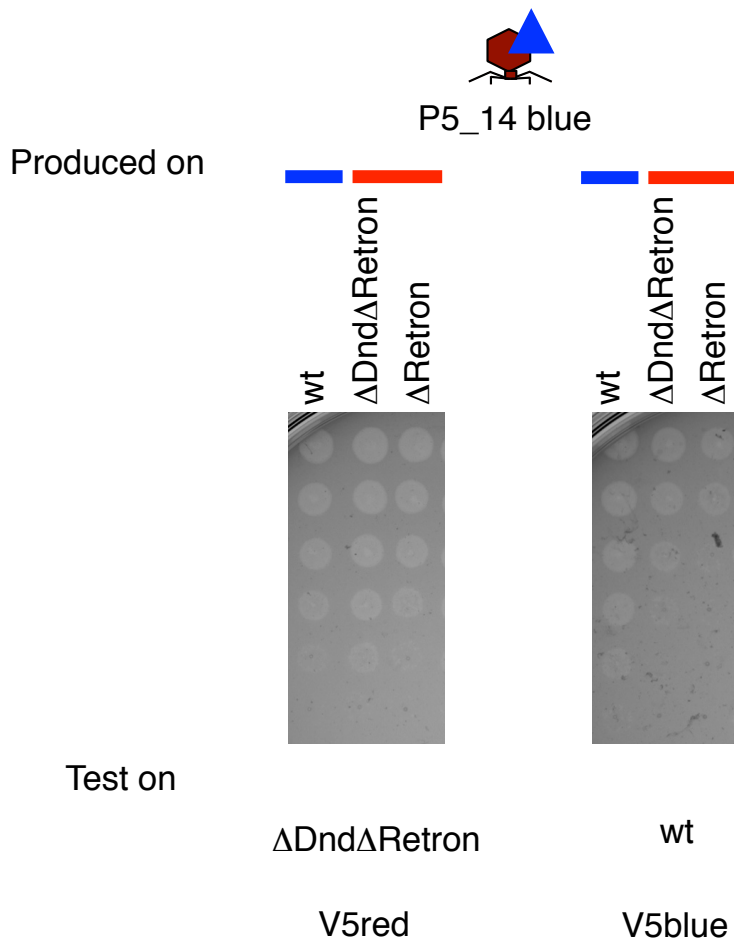
Figure S12. P5_14 blue phages propagated in V5red derivatives are still able to kill the V5blue. A blue phage (66E30.1) was produced in its V5blue original wild type (wt) host (30_P_66) or in V5red (29_O_45) derivatives lacking the Dnd and the retron defence systems ( \Delta Dnd \Delta Retron) or only the retron ( \Delta Retron). Tenfold dilutions of each progeny were spotted on the indicated vibrios strains. When produced in V5red mutants, the blue phage was still able to infect its original V5blue host although at a higher MOI than when produced from the V5blue strain. Experiment was performed twice and images are representative of two independent experiments.
