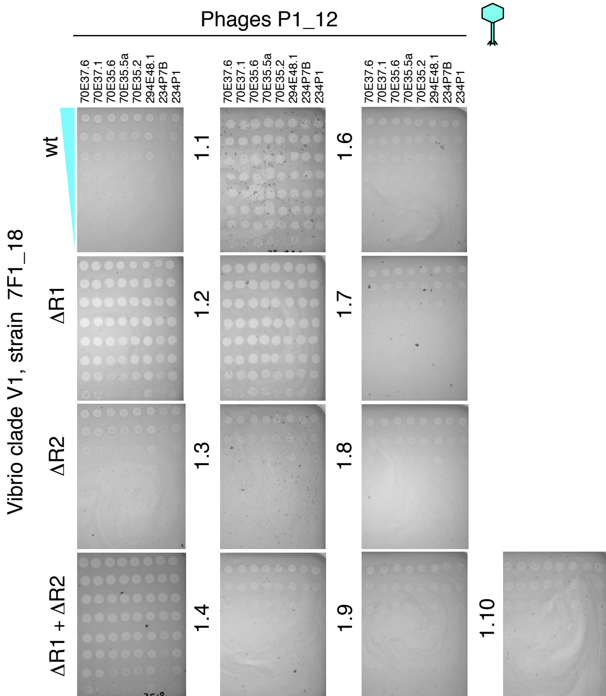
Figure S7. Changes in susceptibility to phage killing observed for phage-defence region deletions or gene inactivation in one strain (7F1_18) of vibrio clade V1 and phage from cluster P1_12. Tenfold dilutions of phage from cluster P1_12 were spotted on the strain 7F1_18 wild type and derivatives ( \Delta R1 , \Delta R2 for complete deletion of strain specific region R1 and R2; 1.1 to 1.10 for gene inactivation in R1 after integration of a suicide vector). Images are representative of two independent experiments.
