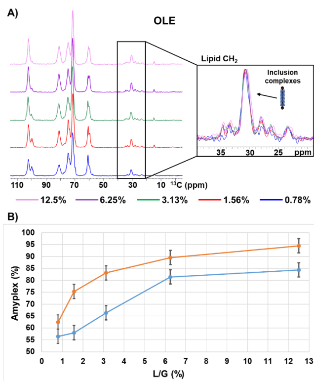
Figure 1. A) ^{13}\text{C} NMR spectra recorded on 50% (w/w) hydrated oleic acid (OLE) / amylose samples obtained with an initial lipid to glucose molar ratio of 0.78% (blue), 1.56% (red), 3.13% (green), 6.25% (purple) and 12.5% (pink). B) Percentage of amylose complexed with palmitic (blue) and oleic (orange) acids in NMR samples (%Amyplex) as a function of the initial L/G molar ratio.
