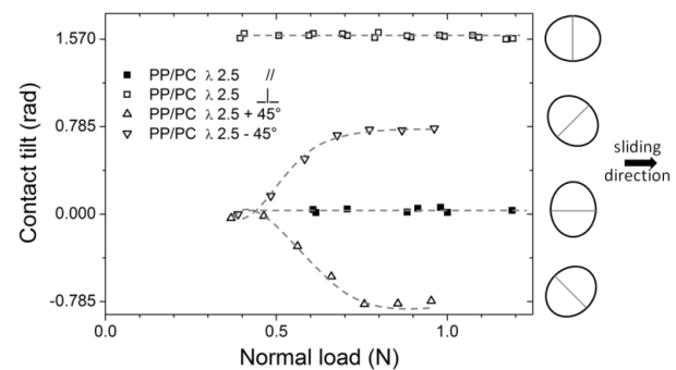
Figure 1: Evolution of the contact tilt of the elliptical contact as a function of normal load and sliding direction.
