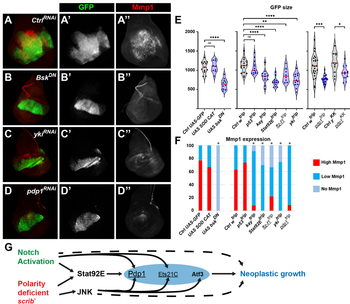
Fig. 4. Neoplastic growth is mediated by an AP-1/Stat/Yki/Ftz-f1 module and by a diverse network of bZIP transcription factors, including Pdp1.
