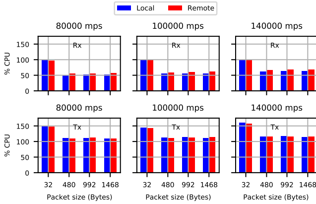
Fig. 3. CPU consumption for A_{Eth}^0 versus A_{Eth}^1 on Ethernet.
