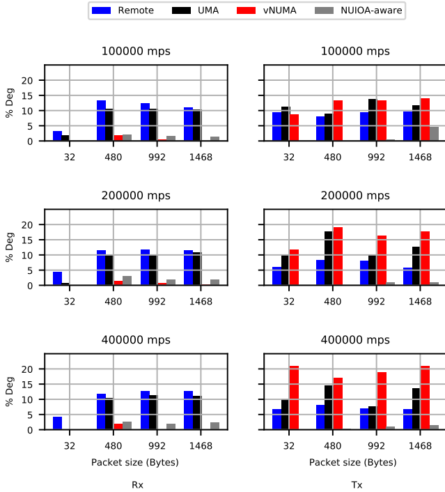
Fig. 7. Sockperf latency evaluation on InfiniBand networking.
