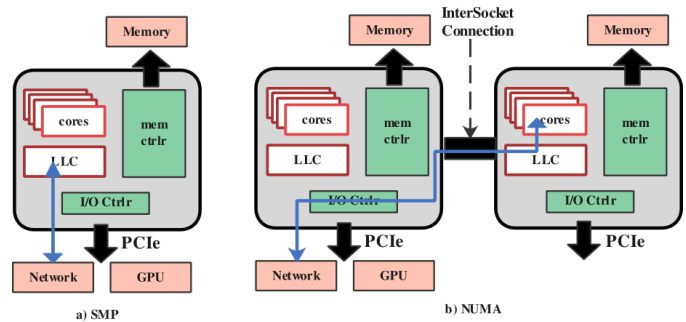
Fig. 1. I/O in a server based on a) UMA (i.e. non-NUMA) architecture; b) NUMA architecture.
