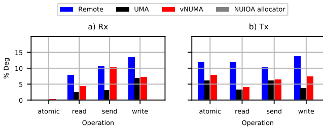
Fig. 11. Perfest evaluation results.
