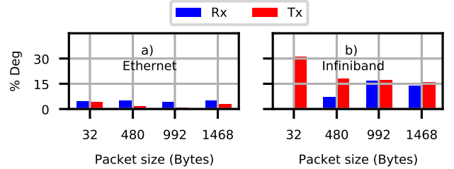
Fig. 4. Socket-interconnect impact on Rx/Tx bandwidth.
