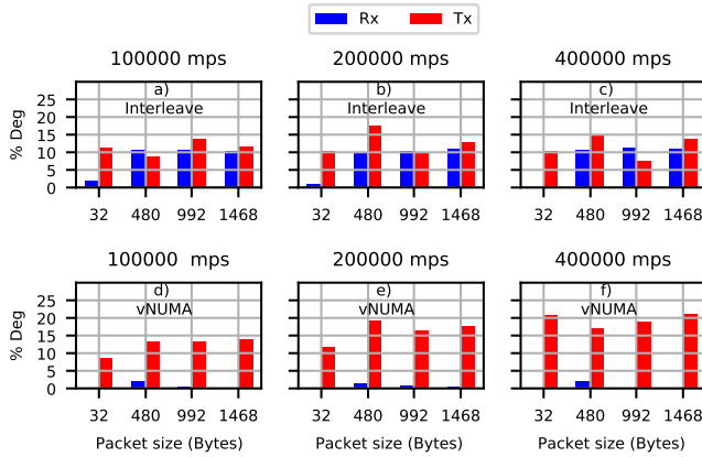
Fig. 5. Impact of interleaved ( U_{Ib}^{0,1} ) and vNUMA ( vN_{Ib}^{0,1} ) configurations on Sockperf latency compared to the reference A_{Ib}^0 .
