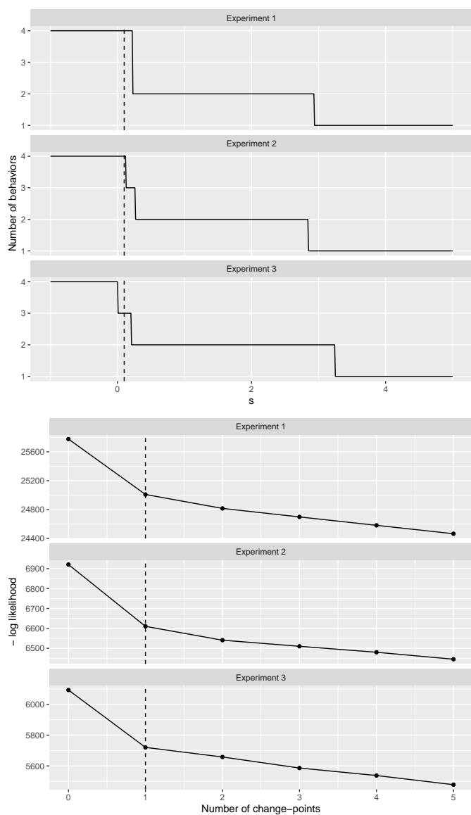
Fig. 6: Choice of the number of change-points.
