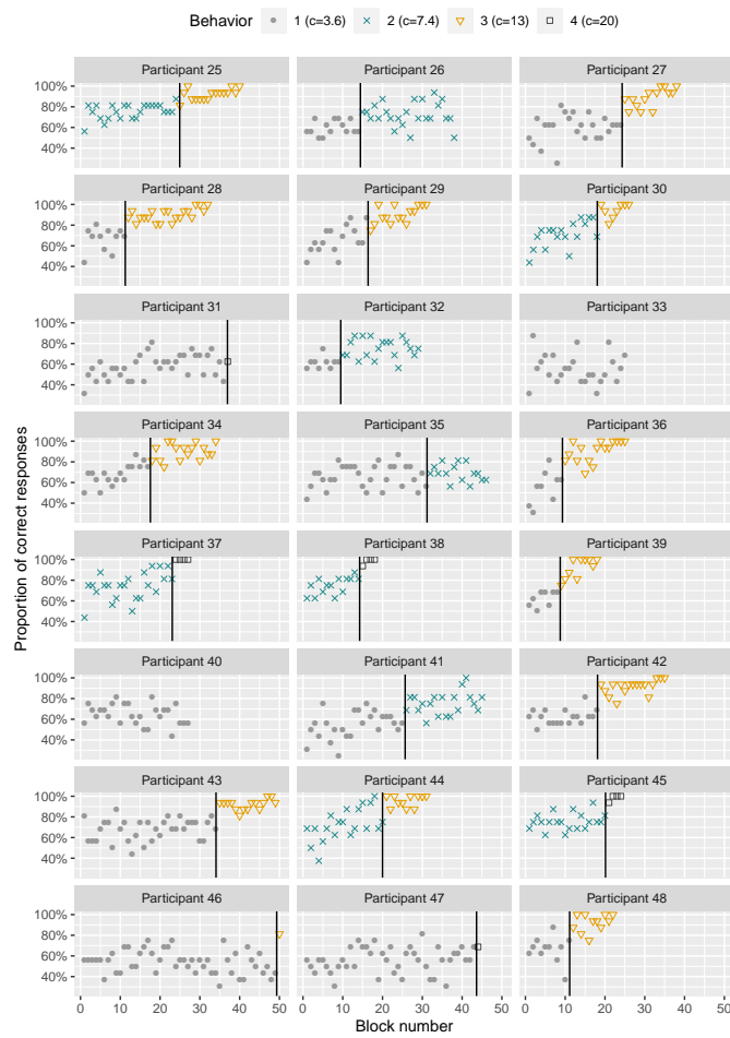
Fig. 13: Result of the application of the segmentation/clustering technique with P = 4 behaviors and K = 1 change-point to Experiment 2.
