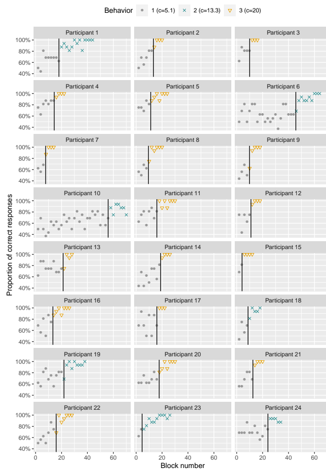
Fig. 14: Result of the application of the segmentation/clustering technique with P = 3 behaviors and K = 1 change-point to Experiment 3 (participants 1-24).
