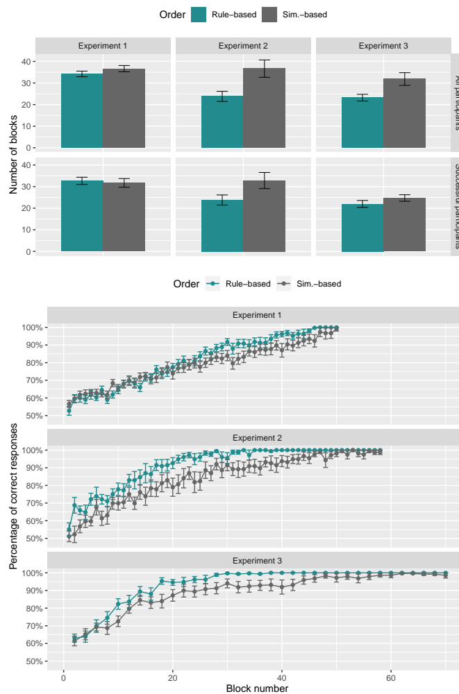
Fig. 9: Participants' learning time and progression as a function of presentation order in Experiments 1-3. On the top, average number of blocks taken by participants to meet the learning criterion, as a function of presentation order. Graphs showing all participants were plotted separately from the ones with successful participants alone. The term "successful" participants refers to those individuals who met the learning criterion. On the bottom, average percentage of correct responses among participants within the same presentation order, as a function of block number. In Experiment 3, only performance across random blocks are plotted.
