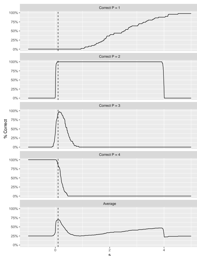
Fig. 1: Numerical simulations for tuning the parameter s (choice of the number of behaviors). The graph shows the percentage of time that the method finds the correct number of behaviors as a function of s , on simulated data having different numbers of behaviors P (from 1 to 4). We run 50 simulations, for each number of behavior. The values of the sensitivity parameter c associated to each behavior were 15 when P = 1 ; 0.005 and 30 when P = 2 ; 0.005, 13, and 30 when P = 3 ; and 0.005, 7, 14, and 30 when P = 4 . The same sequence of stimuli as in Experiment 2 was used to run the simulations. Data was generated such that each participant was affected by K = 1 change-point (equidistant from participant's first and last blocks). P_{\max} = K_{\max} = 5 . The graph on the bottom shows the percentage of correct response, averaged across the previous graphs ( P from 1 to 4). Dashed lines indicate the selected value for s .
