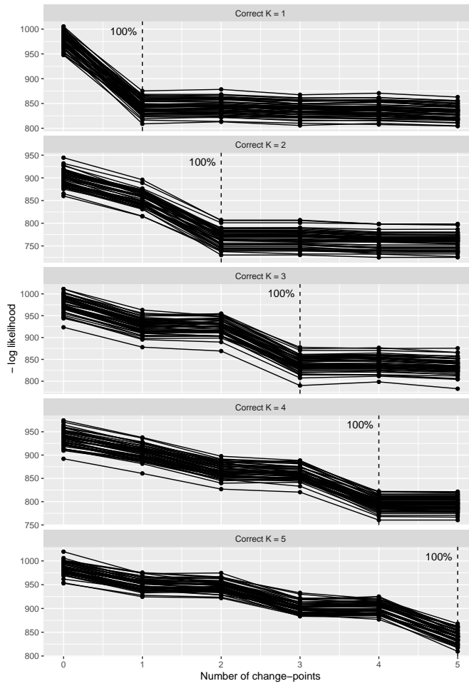
Fig. 3: Numerical simulations when \beta = 10 . The graph shows minus the log likelihood as a function of the number of change-points, on simulated data having different numbers of change-points K (from 1 to 5). For each number of change-points, we run 50 simulations. In each one of the 50 simulations, the method found the same result indicated with dash lines. This means that the method (with \beta = 10 ) found the correct number of change-points 100% of the time, in each case.
