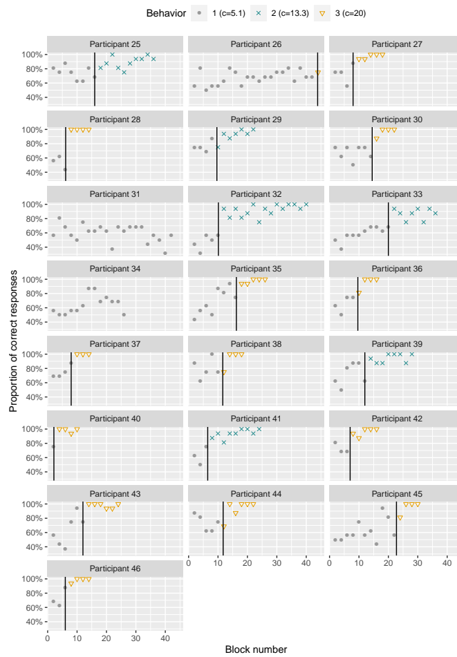
Fig. 14: Result of the application of the segmentation/clustering technique with P = 3 behaviors and K = 1 change-point to Experiment 3 (participants 25-46).
