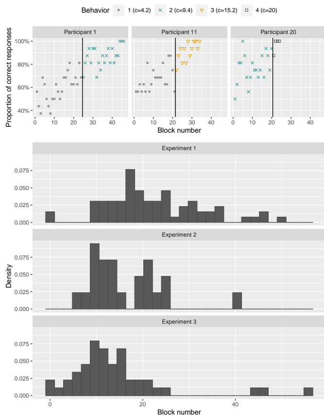
Fig. 8: Results of the application of the segmentation/clustering technique. On the top, visualization of the segmentation/clustering method with P = 4 behaviors and K = 1 change-point to Experiment 2. To make the graph more readable, only 3 participants (Participants 1, 11, and 20) among the 22 were selected. The remaining participants of Experiment 2, as well as those of Experiments 1 and 3 are shown in Appendix B. On the bottom, density function of the coordinate of the change-point (in terms of block number) in Experiments 1-3.
