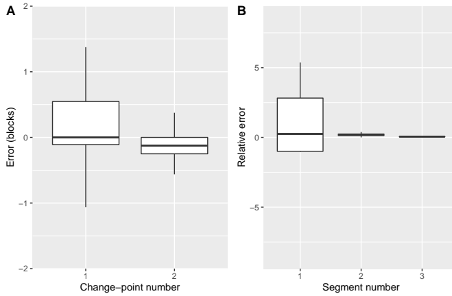
Fig. 4: Error of the segmentation/clustering technique in detecting the coordinate of the change-points (Figure A) and the value of the sensitivity parameter c (Figure B). In A, the error is expressed in terms of number of blocks. In B, the relative error is defined as \frac{c-\hat{c}}{c} . The number of behaviors P was set equal to 3, the number of change-points K was set equal to 2, and the values of the sensitivity parameter c were set equal to 0.2, 7, and 19 for the first, second, and third segment, respectively. The same sequence of stimuli as in Experiment 2 was used to run the simulations. Data was generated such that the K = 2 change-points affecting participants’ progression were equidistant from participant’s first and last blocks.
