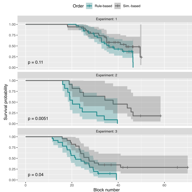
Fig. 10: Kaplan-Meier survival curves for each presentation order as a function of block number in Experiments 1-3. Transparent areas represent the 95% confidence intervals. p -values of the log-rank test assessing the difference between survival curves of participants in the rule-based and similarity-based orders are showed on the bottom-left side of each graph.
