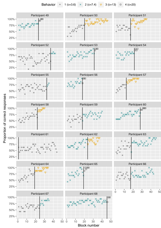
Fig. 12: Result of the application of the segmentation/clustering technique with P = 4 behaviors and K = 1 change-point to Experiment 1 (participants 49-68).
