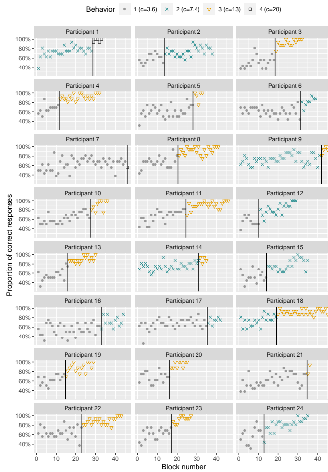
Fig. 12: Result of the application of the segmentation/clustering technique with P = 4 behaviors and K = 1 change-point to Experiment 1 (participants 1-24).
