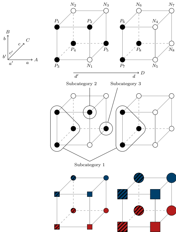
Fig. 5: Illustration of the concept and stimulus items of Experiment 1. On the top, the concept 12_{4[8]} according to Feldman’s classification (Feldman, 2003). Positive stimuli are indicated with black circles, while negative stimuli are indicated with white circles. The notation 12_{4[8]} refers to the fact that this concept is the 12^{th} in the Feldman’s list of 4-dimensional concepts consisting of 8 positive stimuli. In the middle, the substructure made of subcategories in concept 12_{4[8]} . To avoid overburden the figure, only subcategories of the positive stimuli are shown. On the bottom, an example of the 2^4 = 16 stimulus items presented to participants. The items varied along four Boolean dimensions (Shape, Color, Size, and Filling pattern). To make the figure more readable, we illustrated plain and striped items instead of cross-hatched and striped items.
