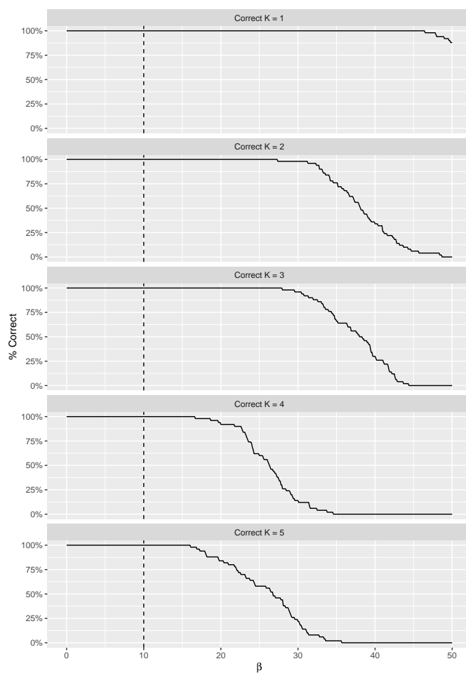
Fig. 2: Numerical simulations for tuning the parameter \beta (choice of the number of change-points). The graph shows the percentage of time that the method finds the correct number of change-points as a function of \beta , on simulated data having different numbers of change-points K (from 1 to 5). We run 50 simulations, for each number of change-points. Data was simulated using two behaviors, P = 2 . The values of the sensitivity parameter c associated to the two behaviors were 0.005 and 15. The same sequence of stimuli as in Experiment 2 was used to run the simulations. Data was generated such that each participant was affected by K change-points (from 1 to 5) equidistant from participant's first and last blocks. K_{\max} = 10 . Dashed lines indicate the selected value for \beta .
