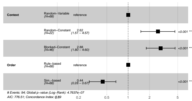
Fig. 11: Results of the application of the Cox model as a function of presentation order and context. In this analysis, Experiments 1-3 have been aggregated together to determine the effect of the three contexts. Hazard ratios and their 95% confidence intervals are showed for each condition in the middle of the graph. Statistical significance of the Wald test is showed for each condition on the right side of the graph.
