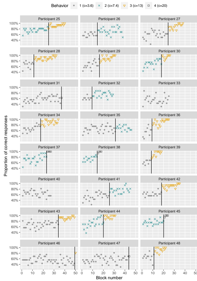
Fig. 12: Result of the application of the segmentation/clustering technique with P = 4 behaviors and K = 1 change-point to Experiment 1 (participants 25-48).
