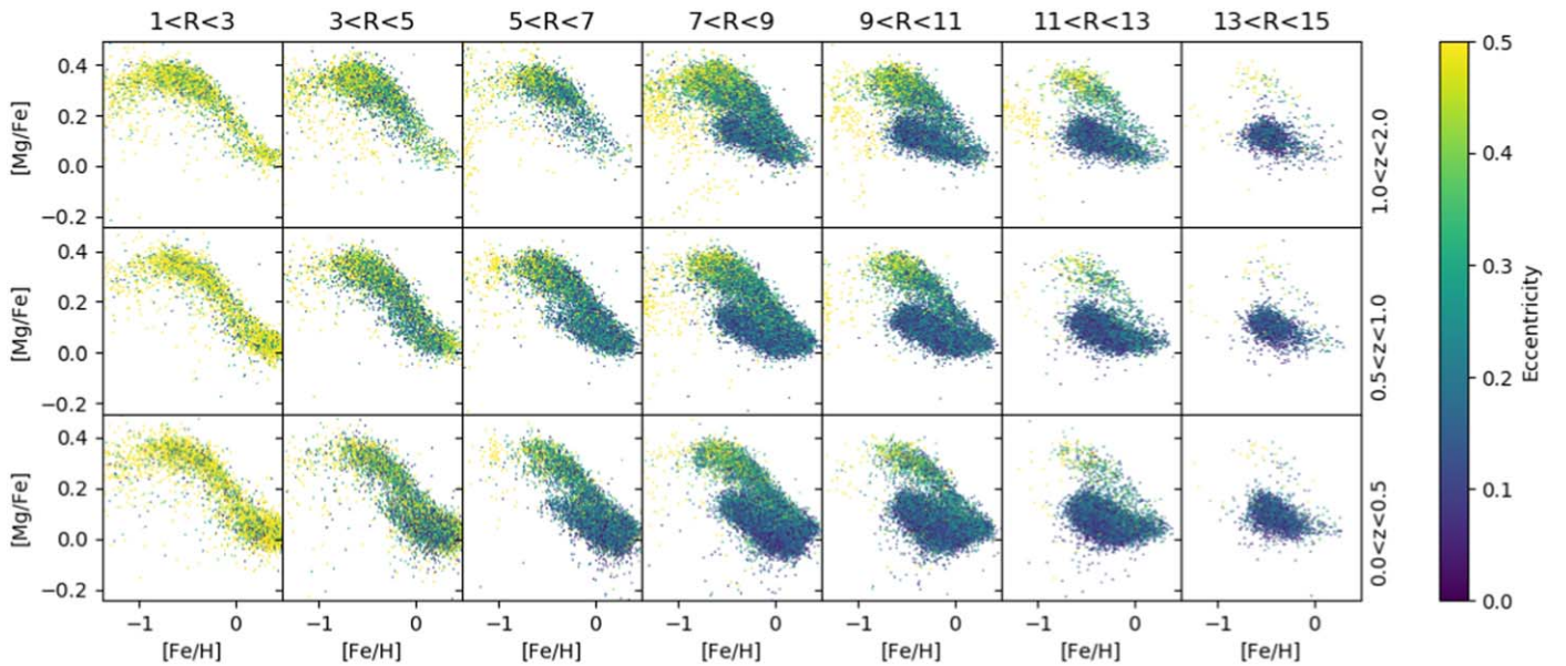
Figure 4. A series of [Mg/Fe] vs. [Fe/H] plots from APOGEE DR17 for different zones in the Milky Way. Distances from the DistMass VAC are used to determine Galactocentric radius ( R_G ) and height above the plane ( z ). Points are color-coded by orbital eccentricities as computed with GalPy (Bovy 2015) using Gaia EDR3 proper motions and APOGEE RVs.
