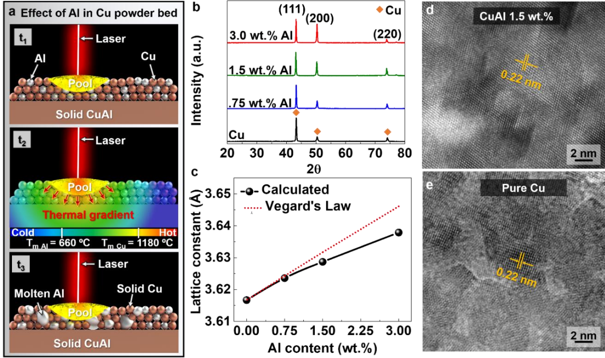
Figure 4. a Illustration of the effect of Al in Cu powder during the 3D printing process, b XRD patterns of the 3D printed samples, c Lattice constant as a function of the Al content, d HR-TEM of 1.5 wt.% Al in Cu, and e HR-TEM of pure Cu.
